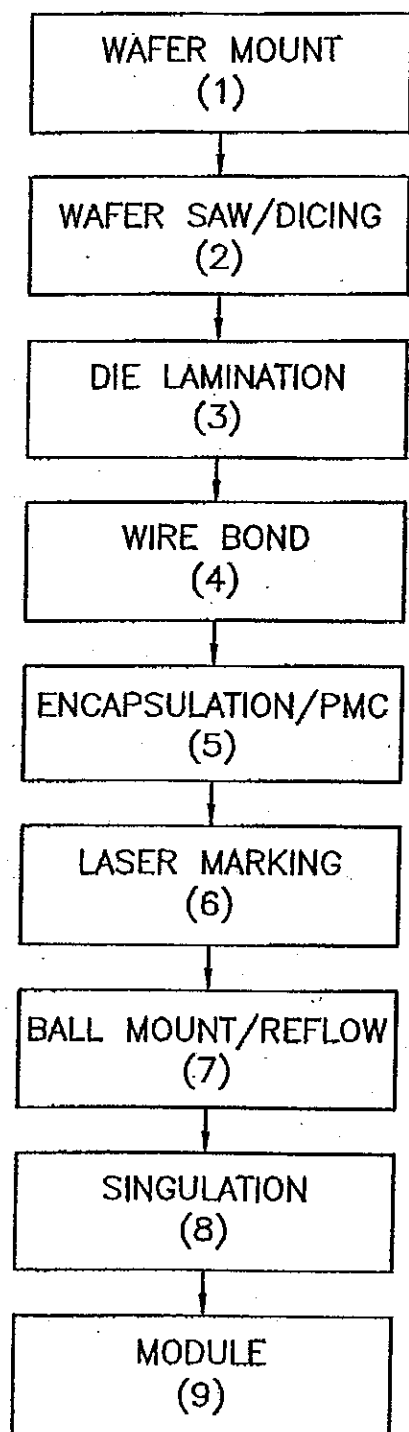
FIGURE 4A (PRIOR ART).
