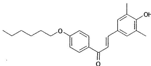
1-[4-hexyloxyphenyl]
