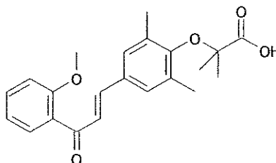
1-[2-methoxyphenyl] 5 -3-[3,5-dimethyl-4-carboxydimethylmethoxyphenyl]prop-2-en-1-one (Compound 6)
