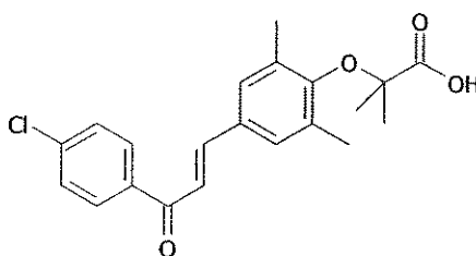
1-[4-chlorophenyl]-3-[3,5-dimethyl-4-carboxydimethylmethoxyphenyl]prop-2-en-1-one (Compound 3)
