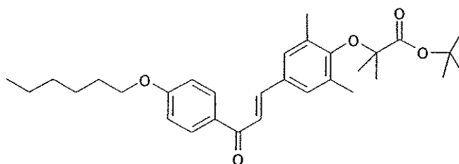
1-[4-hexyloxyphenyl]
