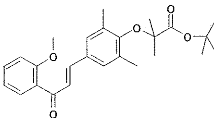
1-[2-methoxyphenyl]-3-[3,5-dimethyl-4-tert-butyloxycarbonyldimethylmethoxyphenyl]prop-2-en-1-one (Compound 5)
