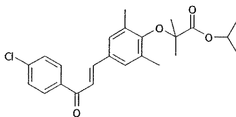
1-[4-chlorophenyl]-3-[3,5-dimethyl-4-carboxydimethylmethoxyphenyl]prop-2-en-1-one
