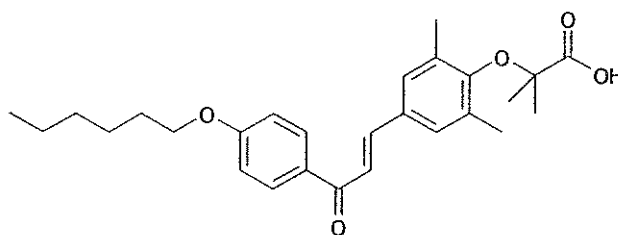
1-[4-hexyloxyphenyl]
