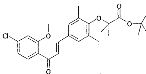
) 1-[2-methoxy-4-chlorophenyl]-3-[3,5-dimethyl-4-carboxydimethylmethoxyphenyl]prop-2-en-1-one
