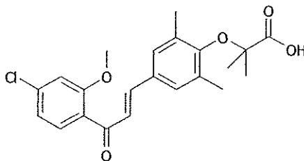
1-[2-methoxy-4-chlorophenyl]
