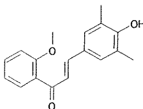
1-[2-methoxyphenyl] -3-[3,5-dimethyl-4-hydroxyphenyl]prop-2-en-1-one (Compound 4)
