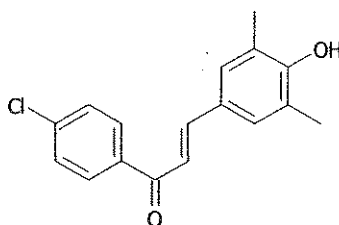
1-[4-chlorophenyl]-3-[3,5-dimethyl-4-hydroxyphenyl]prop-2-en-1-one (Compound 1)
