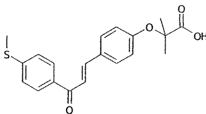
1-[4-carboxydimethylmethoxyphenyl]-3-[4-chlorophenyl]prop-2-en-1-one
