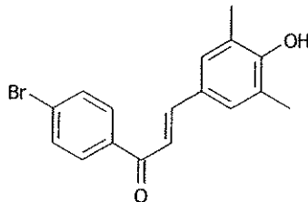
1-[4-bromophenyl]-3-[3,5-dimethyl-4-hydroxyphenyl]prop-2-en-1-one (Compound 16)
