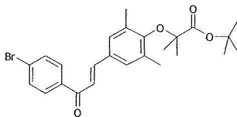
1-[4-bromophenyl]-3-[3,5-dimethyl-4-tert-butylloxycarbonyldimethylmethoxyphenyl]prop-2-en-1-one (Compound 17)
