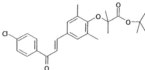
1-[4-chlorophenyl]-3-[3,5-dimethyl-4-tert-butylloxycarbonyldimethylmethoxyphenyl]prop-2-en-1-one (Compound 2)
