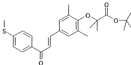
1-[4-methylthiophenyl]-3-[3,5-dimethyl-4-tert-butylloxycarbonyldimethylmethoxyphenyl]prop-2-en-1-one (Compound 8)
