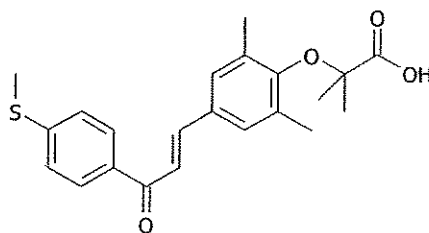
1-[4-methylthiophenyl]-3-[3,5-dimethyl-4-carboxydimethylmethoxyphenyl]prop-2-en-1-one (Compound 9)
