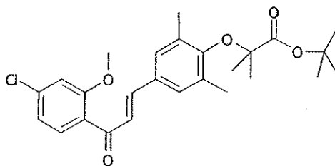
1-[2-methoxy-4-chlorophenyl]
