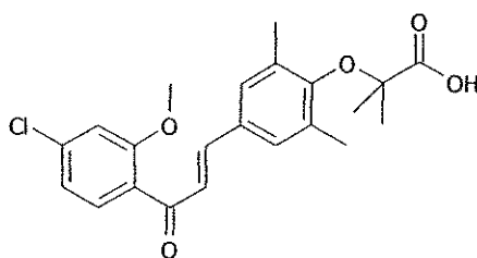
) 1-[2-methoxy-4-chlorophenyl]-3-[3,5-dimethyl-4-carboxydimethylmethoxyphenyl]prop-2-en-1-one
