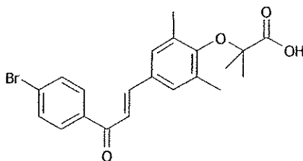
1-[4-bromophenyl]-3-[3,5-dimethyl-4-carboxydimethylmethoxyphenyl]prop-2-en-1-one (Compound 18)
