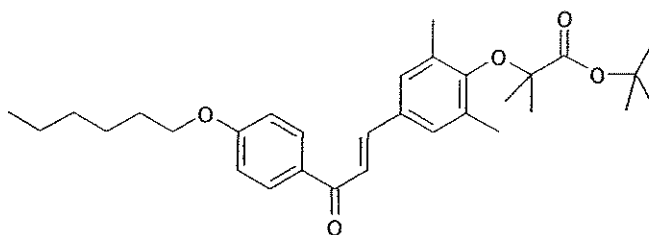
5 1-[4-hexyloxyphenyl]-3-[3,5-dimethyl-4-carboxydimethylmethoxyphenyl]prop-2-en-1-one
