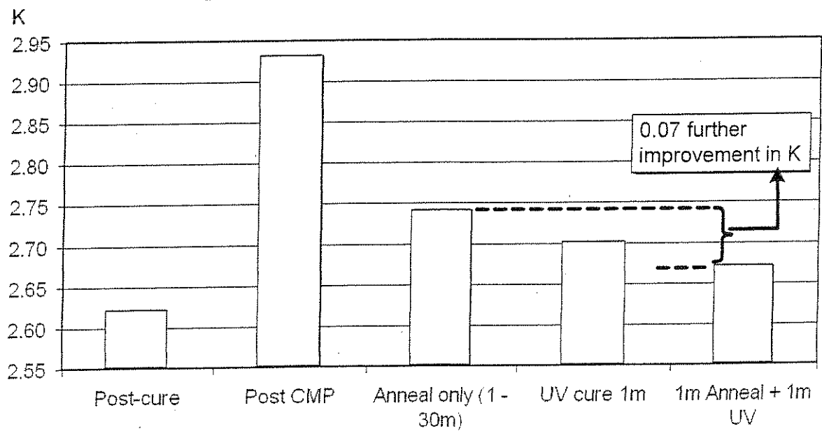
Impact of UV cure on Post-CMP K recovery
