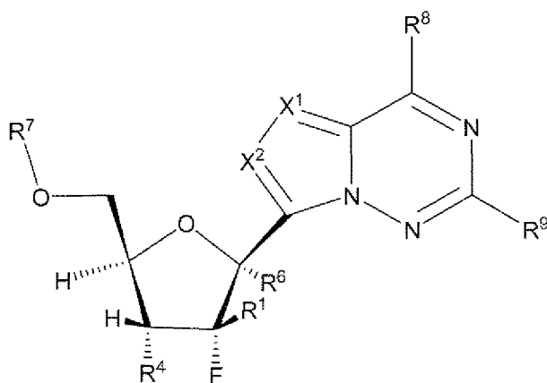
Formula III
