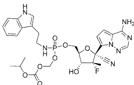
Compound 26
