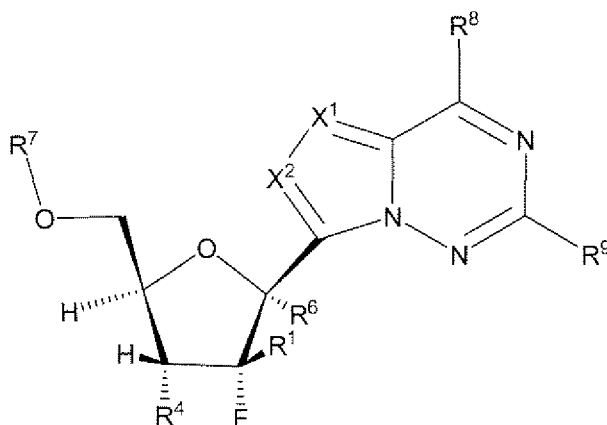
Formula III
