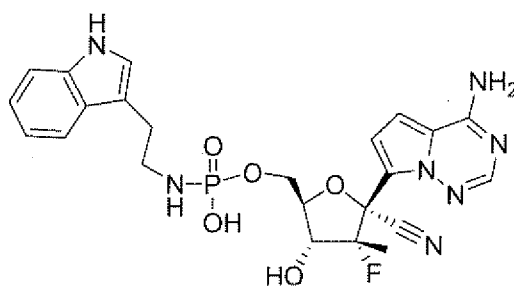
Compound 22
