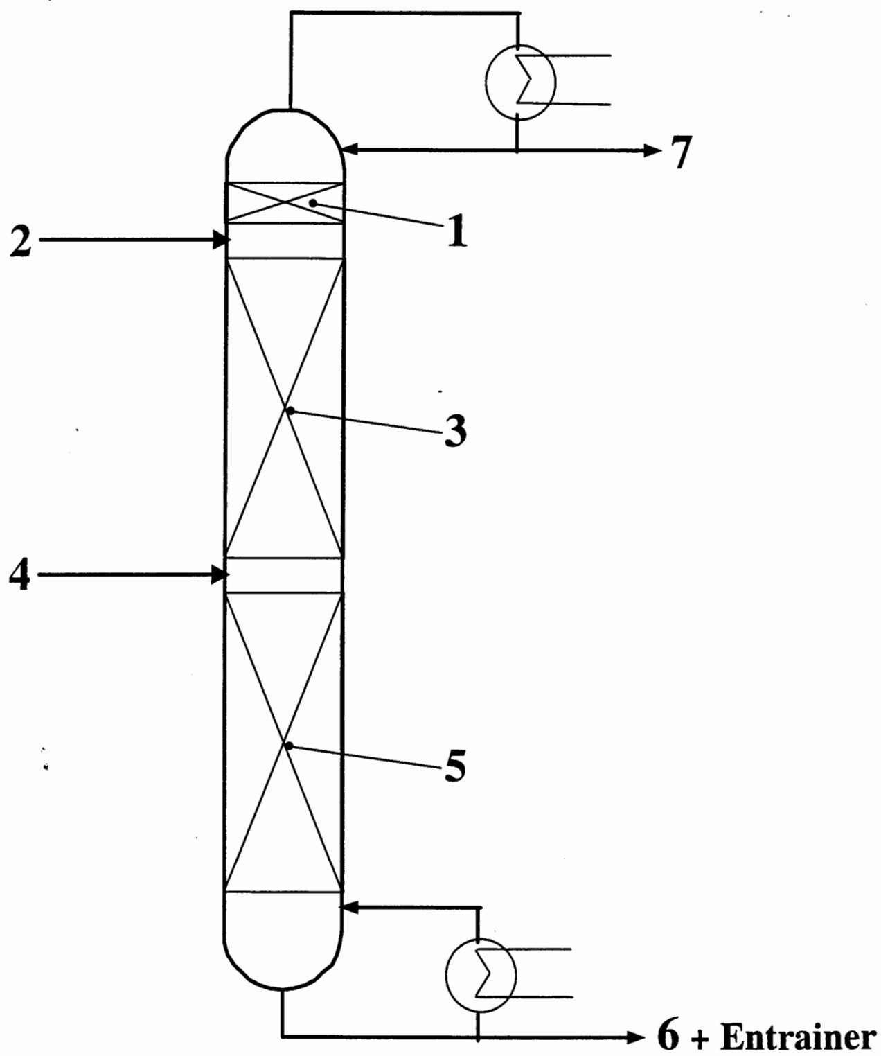
Figure 1: Embodiment of the extractive rectification system
