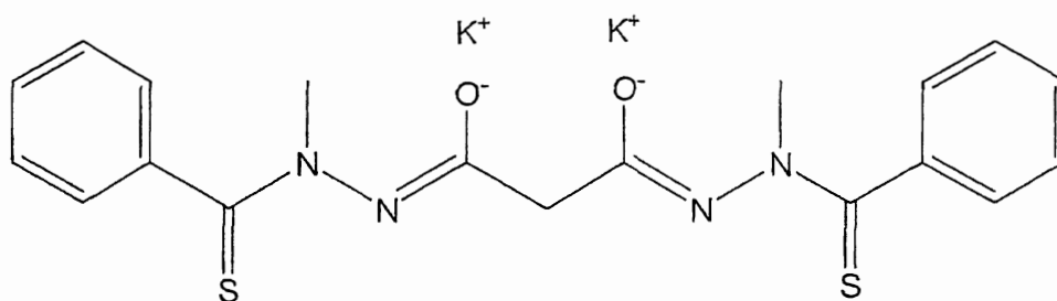
Compound (2)
