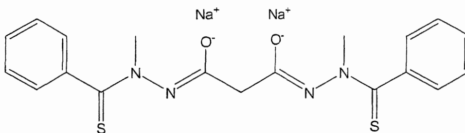
Compound (1)
