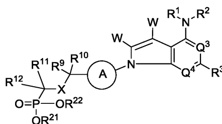
Formula (V);
