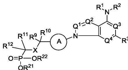
Formula (III);
