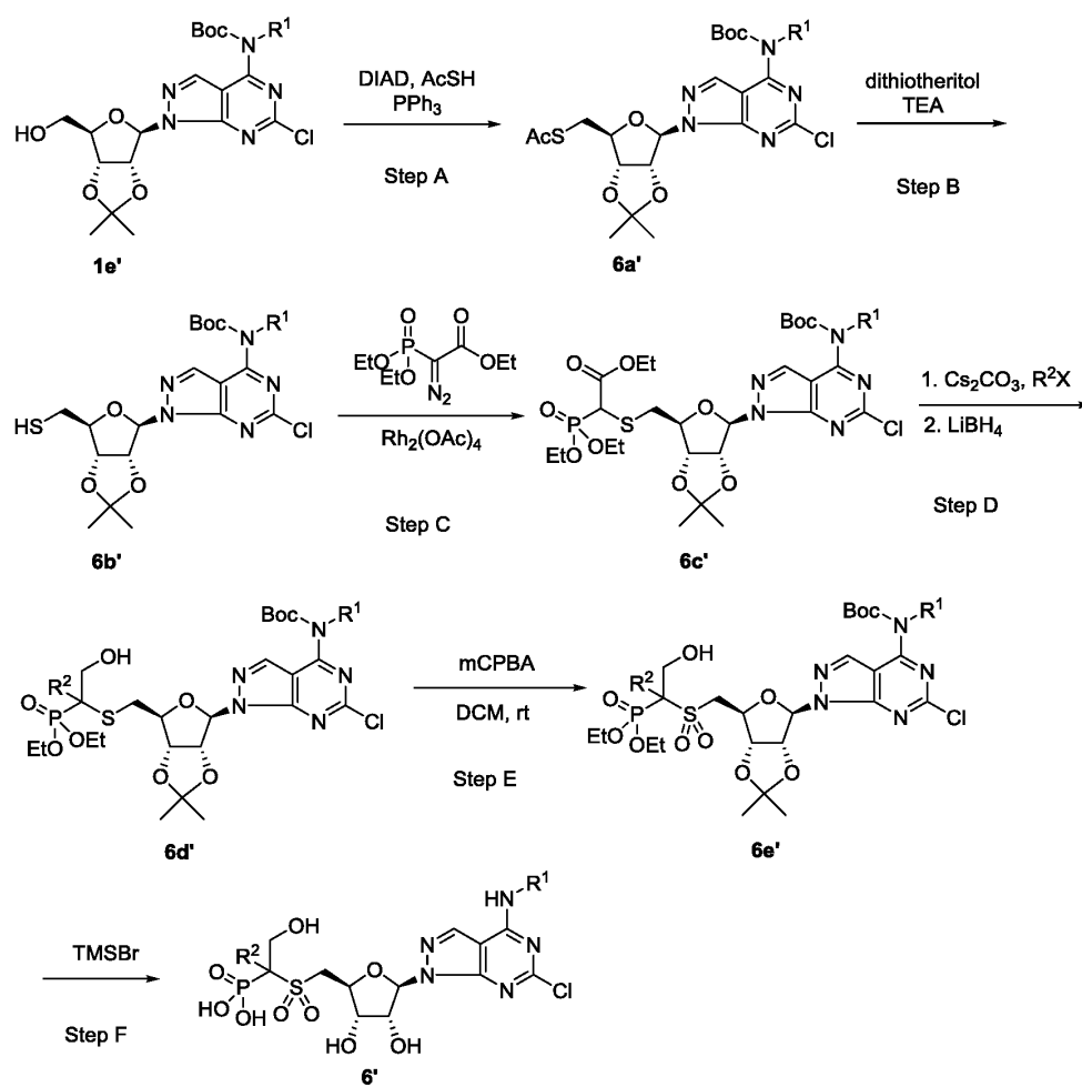
Scheme 7
