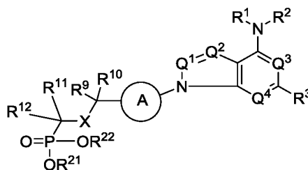
Formula (II);
