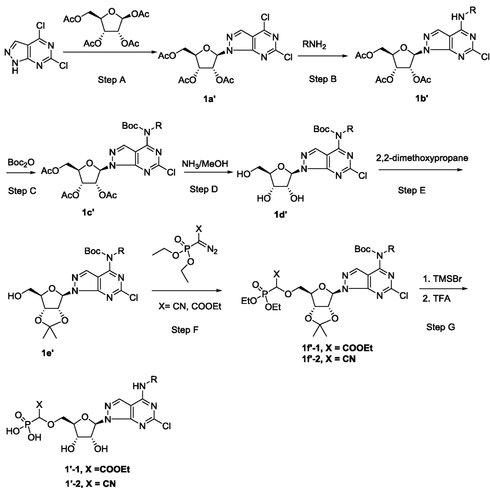
Scheme 1
