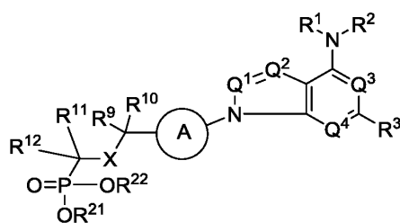
Formula (II);
