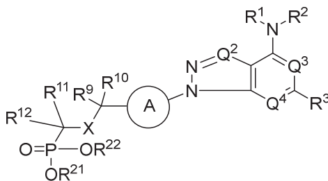
Formula (IV);
