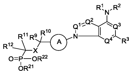
Formula (II);
