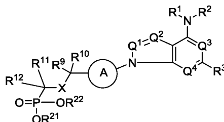
Formula (III);
