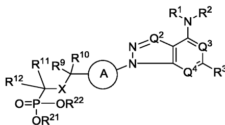
Formula (IV);
