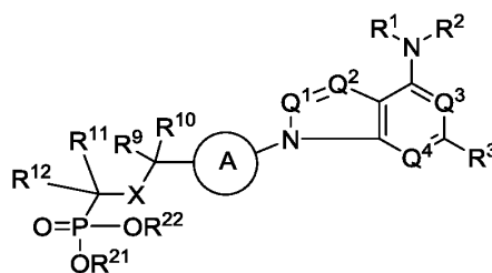
Formula (III);
