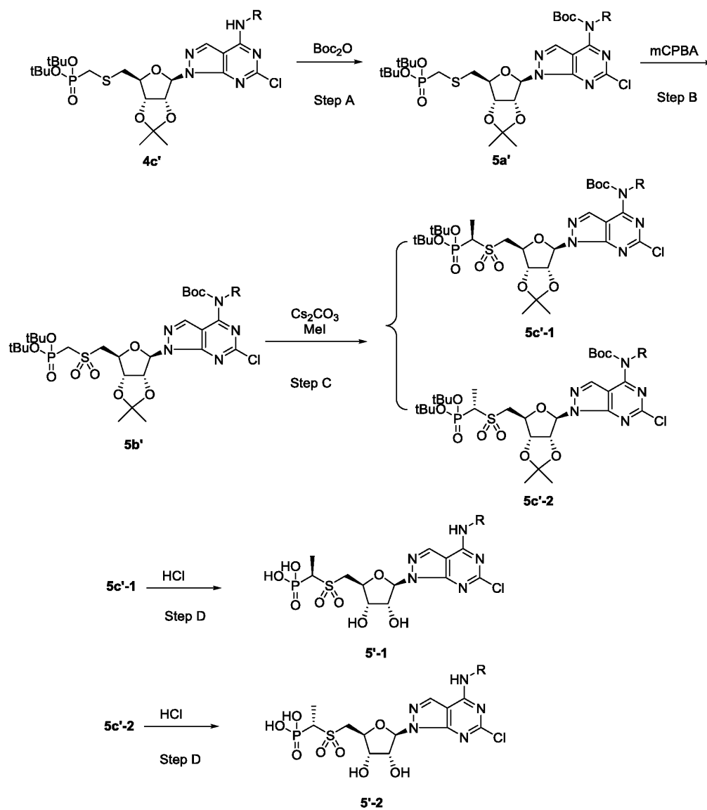
Scheme 6
