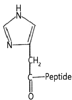
Imidazoacetyl (CA)-GLP-2
