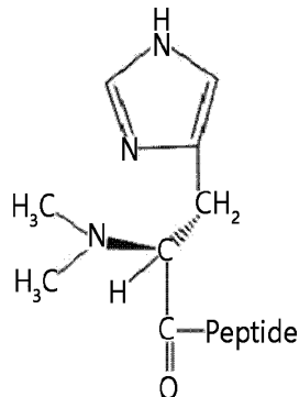
Dimethyl-histidyl (DM)-GLP-2
