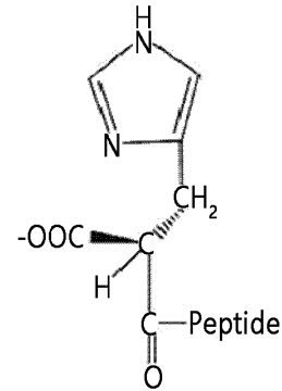
Beta-carboxyl-imidazopropionyl (CX)-GLP-2
