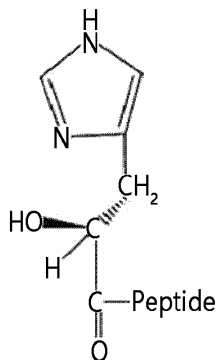
Beta-hydroxy-imidazopropionyl (HY)-GLP-2
