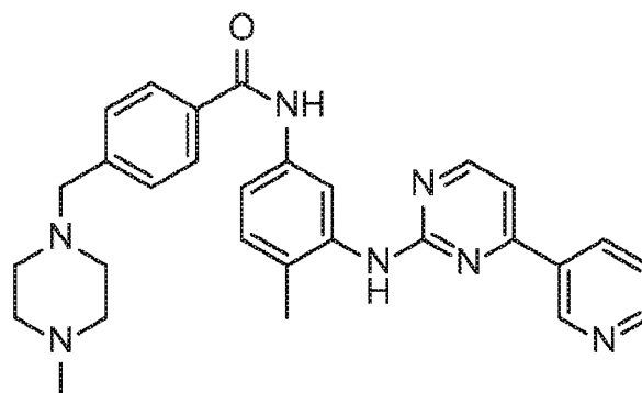
Imatinib
