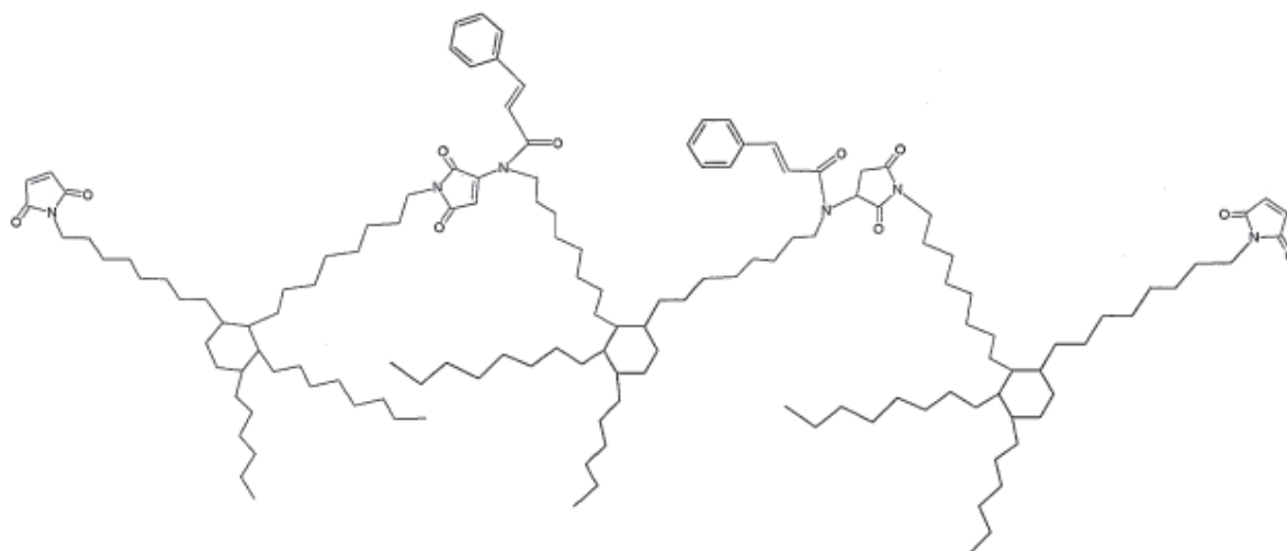
[Chemical Formula 7]
