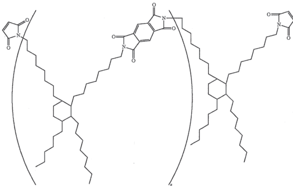
[Chemical Formula 4]
