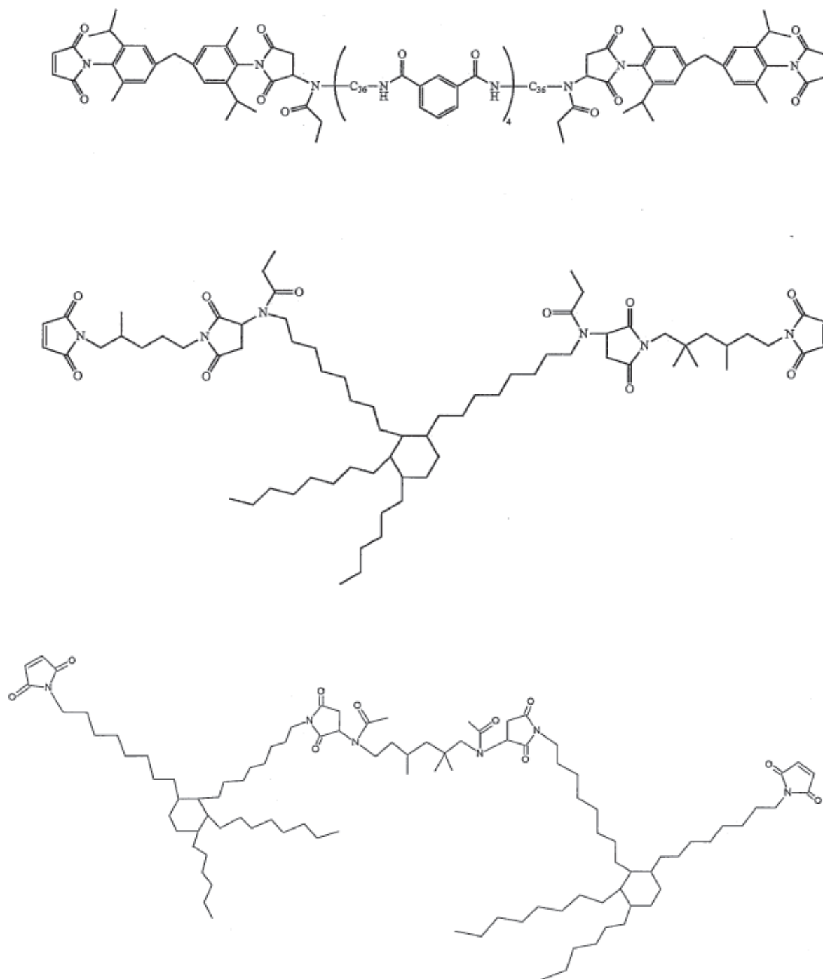
[Chemical Formula 8]
