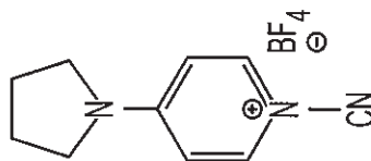
1-CYANO-4-PYRROLIDINOPYRIDINIUM TETRAFLUORBORATE (CPIP OR CPPT)
