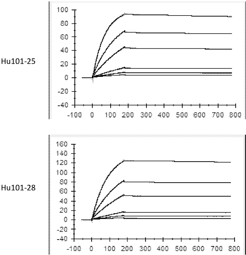
Recombinant CD73 binding by SPR
