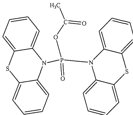
1-(diphenothiazin-10H-yl-phosphinyl)ethanone (XIX)
