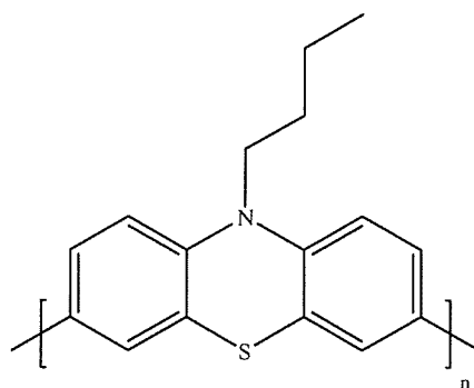
polybutylphenothiazine (XIV)
