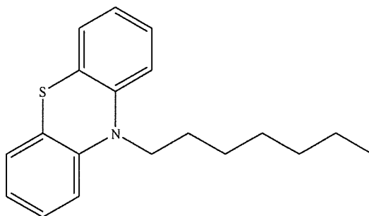
10H-heptylphenothiazine (VIII)
