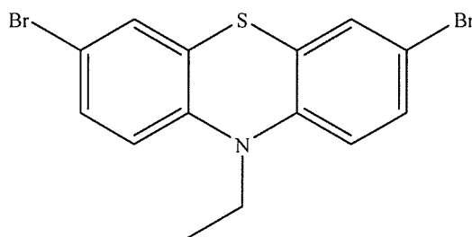
3,3'-dibromo-10H-ethylphenothiazine (V)
