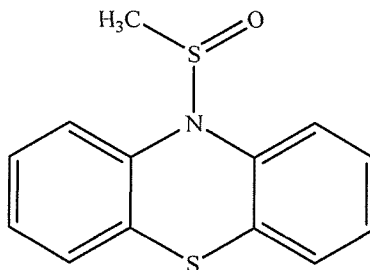
10H-methanesulfinylphenothiazine (XVII)
