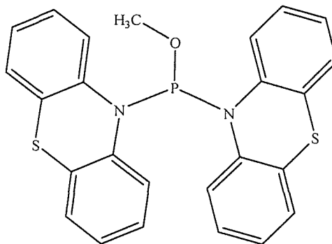
diphenothiazin-10H-yl-methylphosphite (XVIII)
