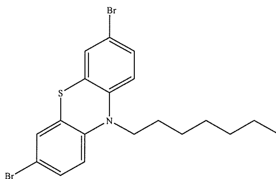
3,3'-dibromo-10H-heptylphenothiazine (IX)
