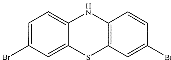
3,3'-dibromophenothiazine (XII)
