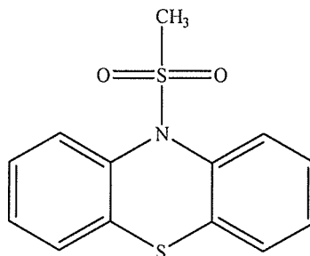
10H-methylsulfonylphenothiazine (XVI)
