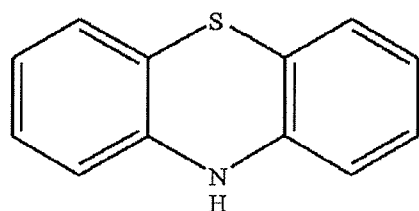
Phenothiazine (I)
