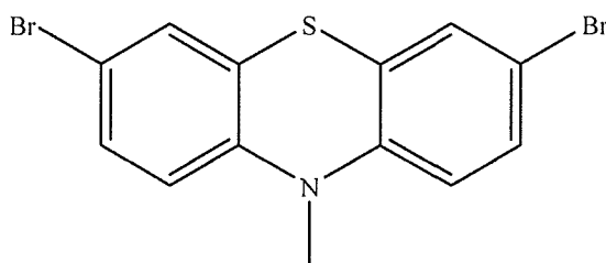
3,3'-dibromo-10H-methylphenothiazine (III)
