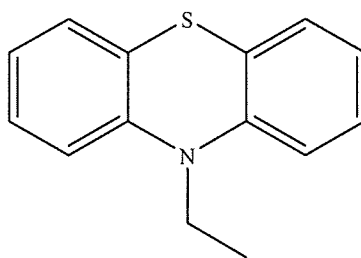
10H-ethylphenothiazine (IV)
