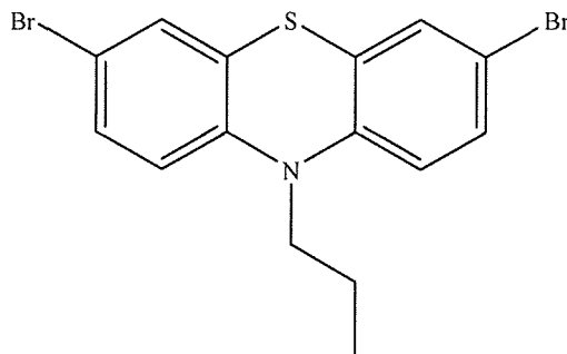
3,3'-dibromo-10H-propylphenothiazine (VII)
