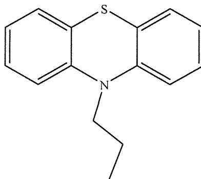
10H-propylphenothiazine (VI)
