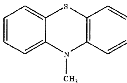
10H-methylphenothiazine (II)
