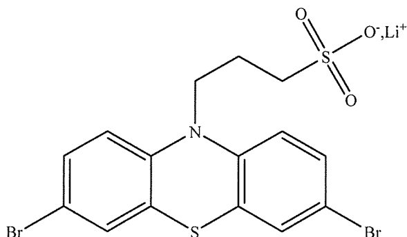
3,3'-dibromo-10H-(lithium propanesulfonate)-phenothiazine ( XIII )
