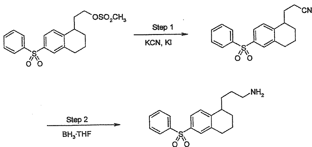
SCHEME O
