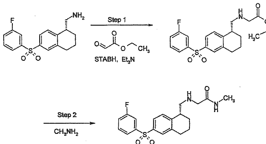
SCHEME AA
