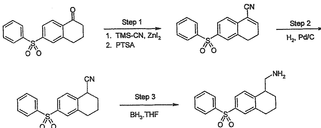
SCHEME F
