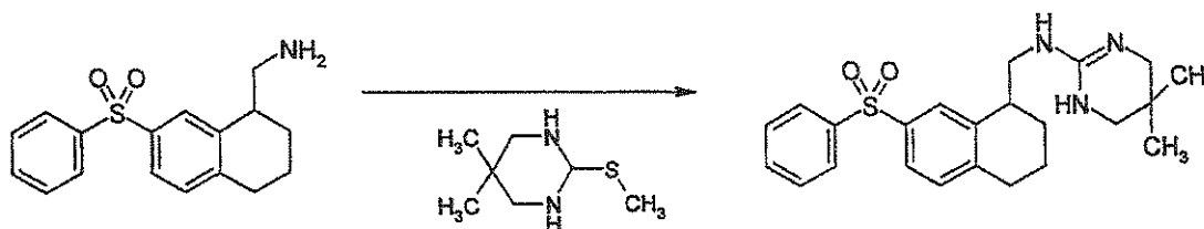
SCHEME K
