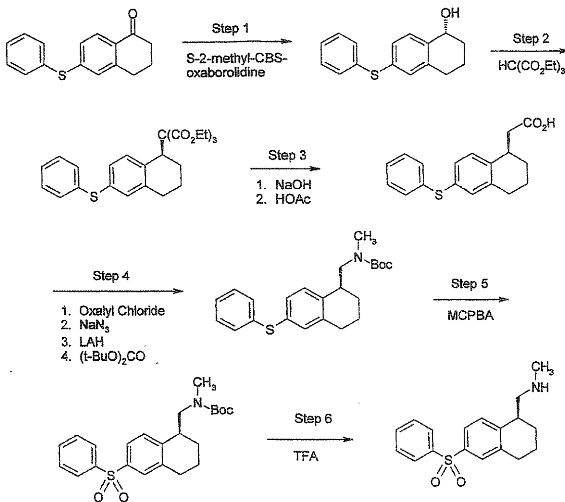
SCHEME R
