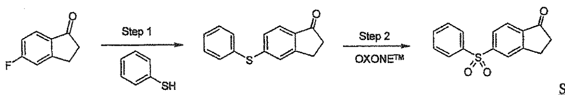
SCHEME E
