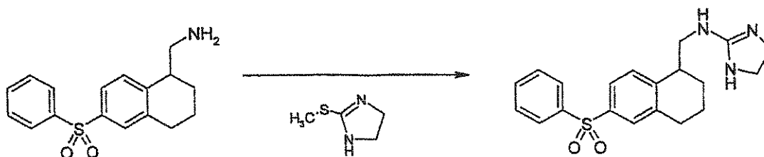
SCHEME J
