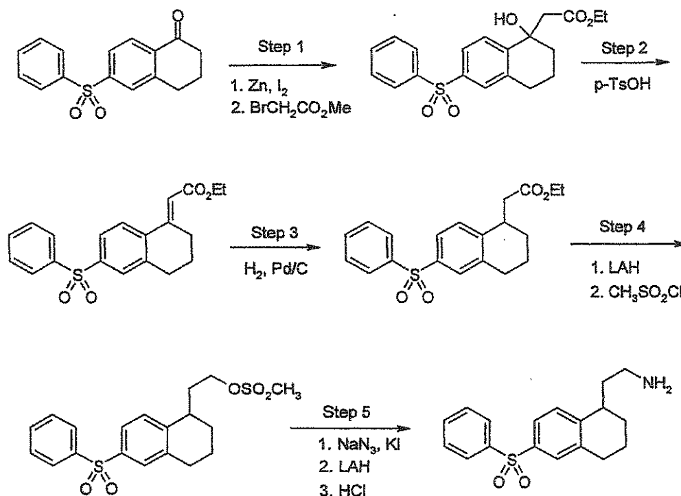
SCHEME L
