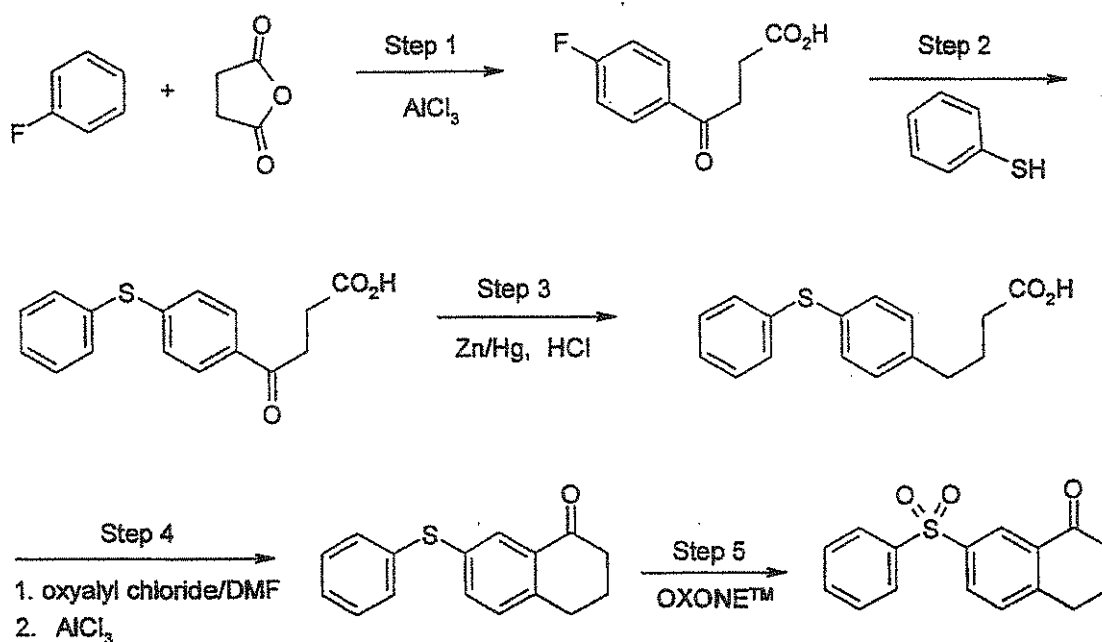
SCHEME D
