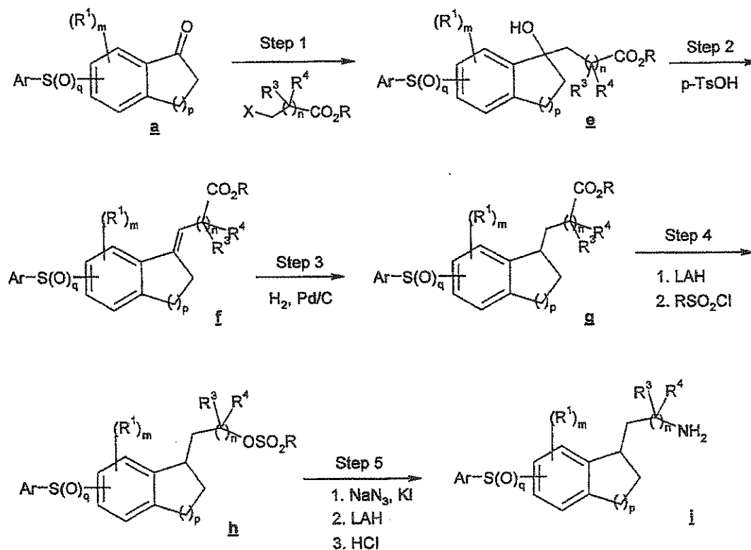
SCHEME B
