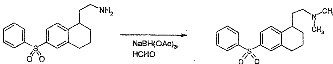
SCHEME N
