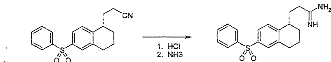
SCHEME P
