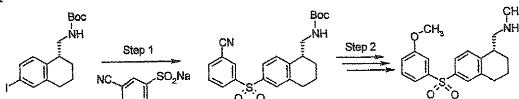
SCHEME U
