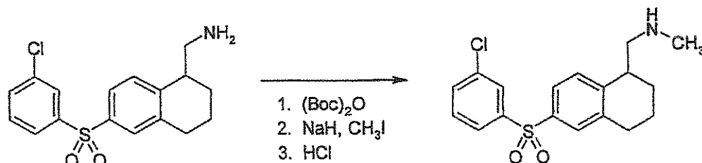
SCHEME G
