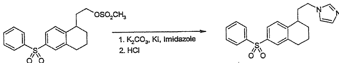
SCHEME Q
