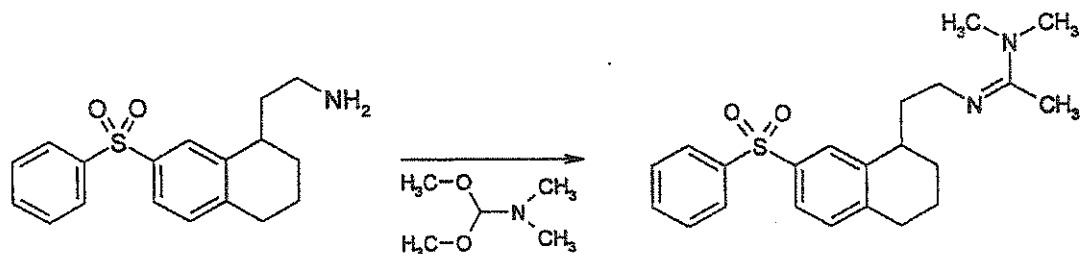
SCHEME M
