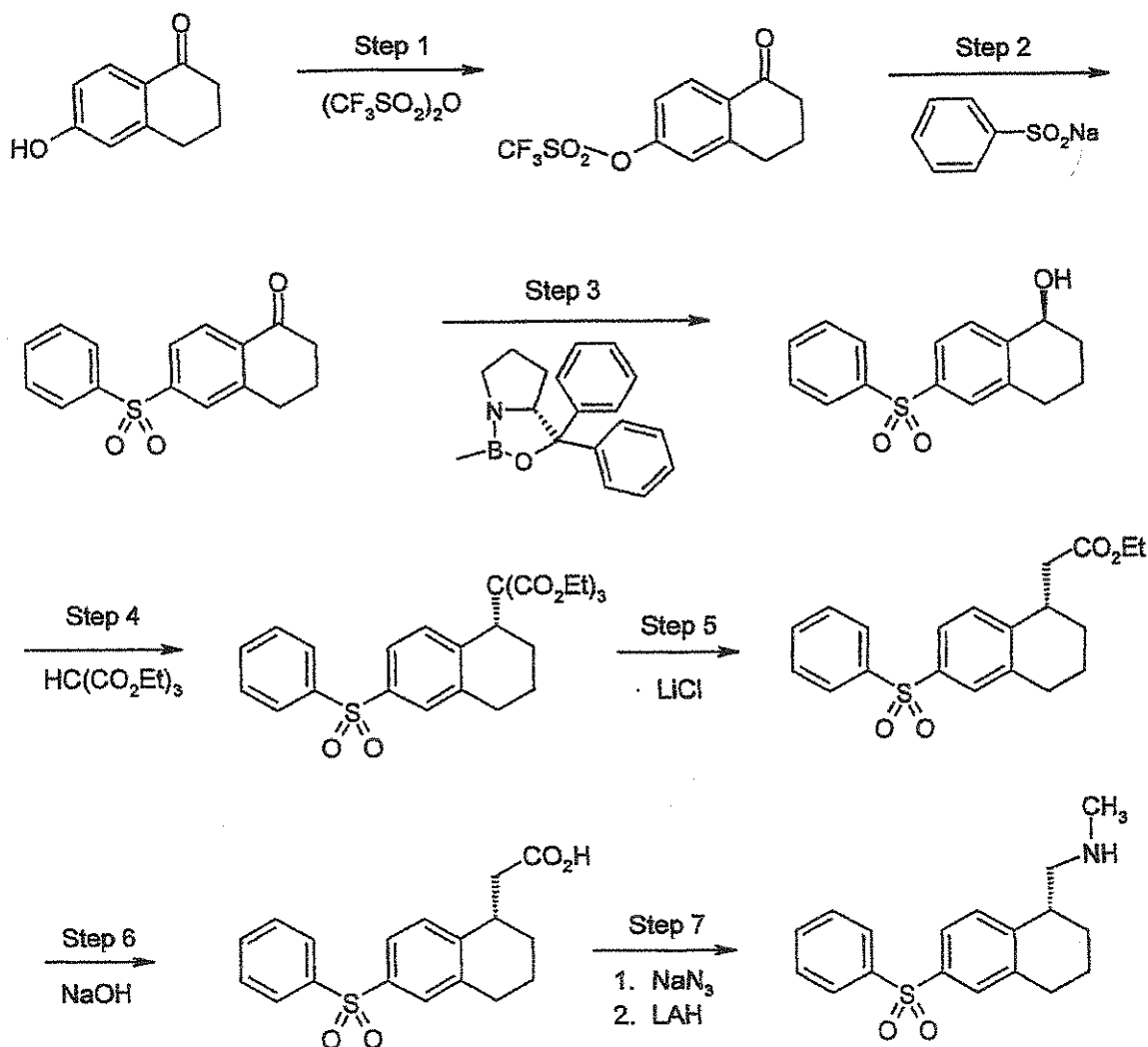
SCHEME S
