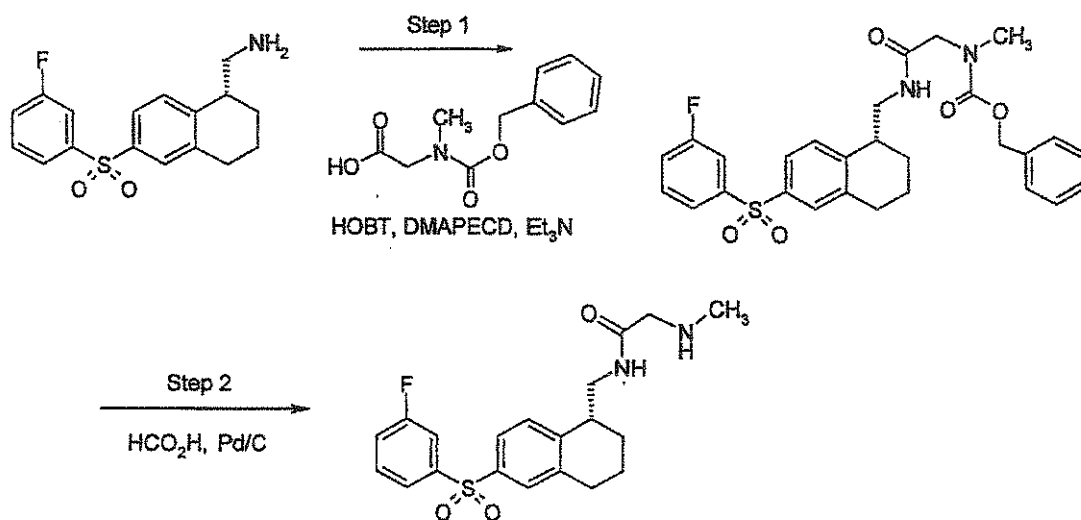
10 SCHEME Z
