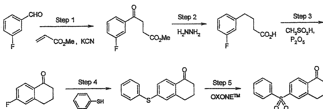
SCHEME C
