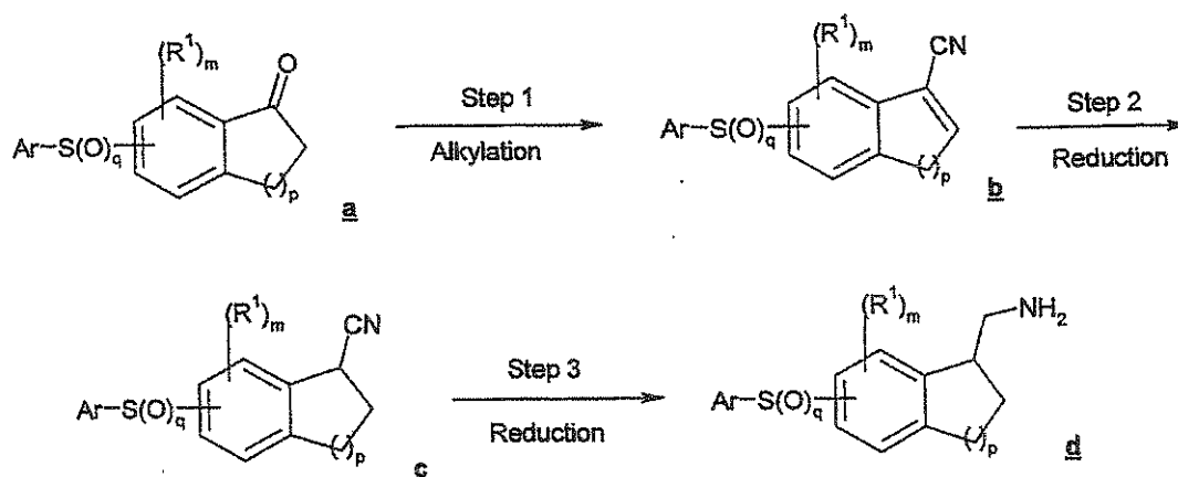
SCHEME A
