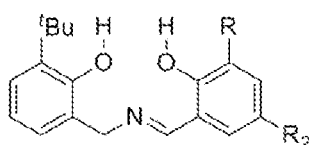
Structure X
