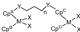
Formula 2
