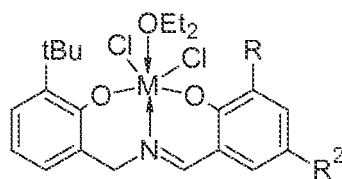
Structure XIV
