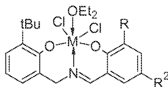
Structure XIV
