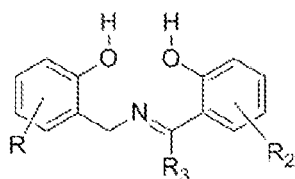
Structure IX
