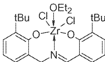
Structure X
