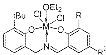
Structure XIV
