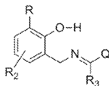
Structure I
