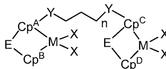
Formula 4
