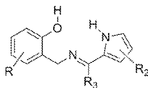
Structure XI
