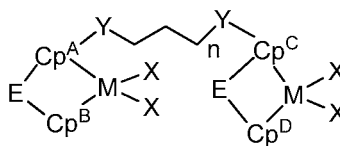
Formula 4
