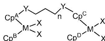
Formula 2
