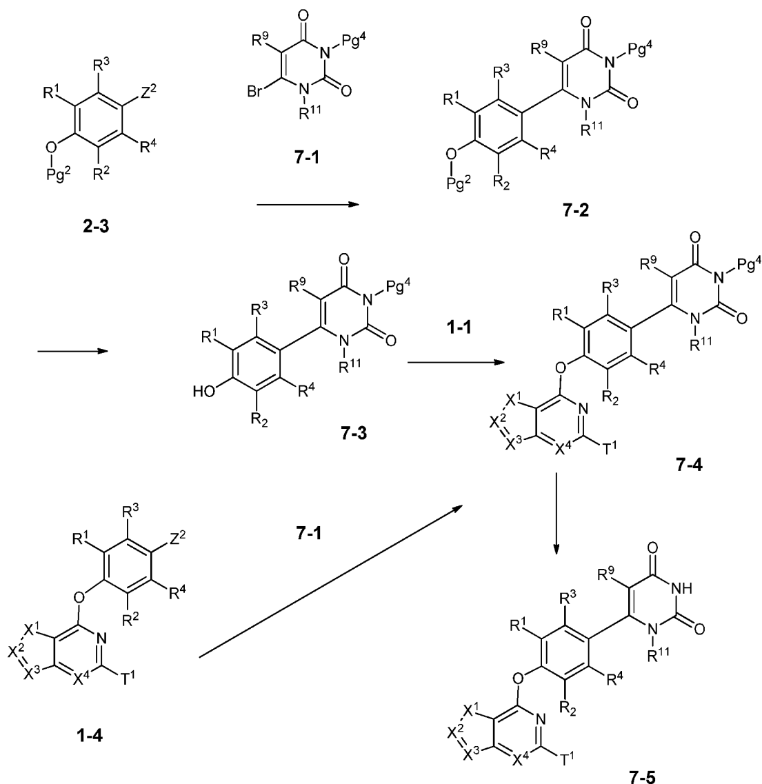
Scheme 7
