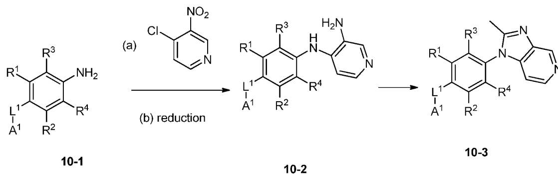
Scheme 10
