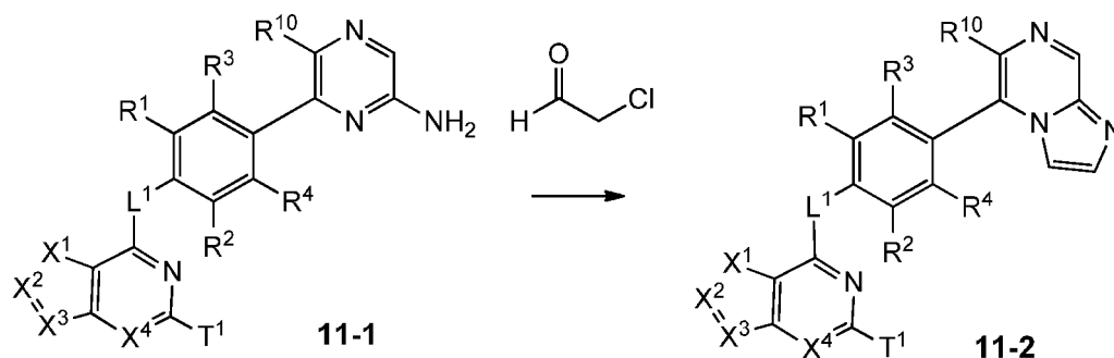
Scheme 11
