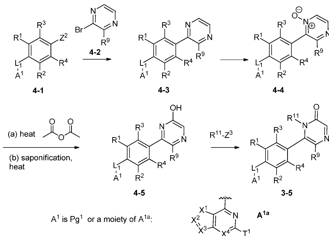
Scheme 4
