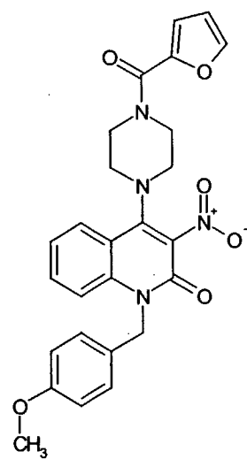
Compound 271
