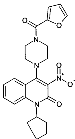
Compound 323
