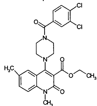
Compound 73
