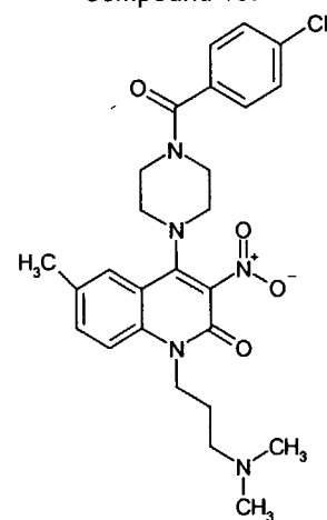
Compound 187
