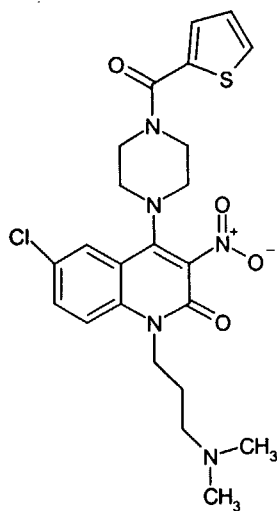
Compound 202
