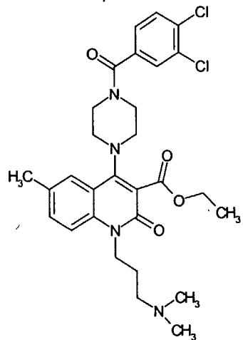
Compound 154
