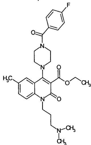
Compound 113
