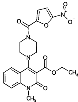
Compound 257
