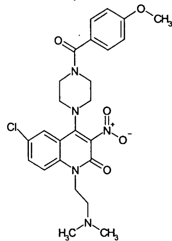
Compound 211
