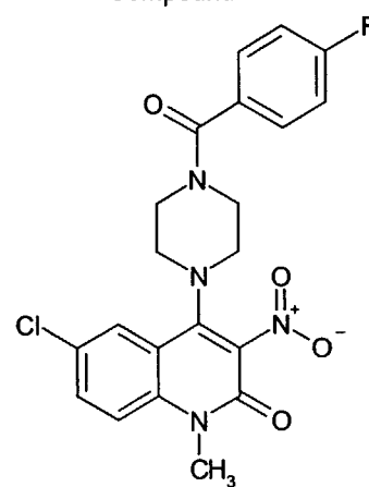
Compound 127
