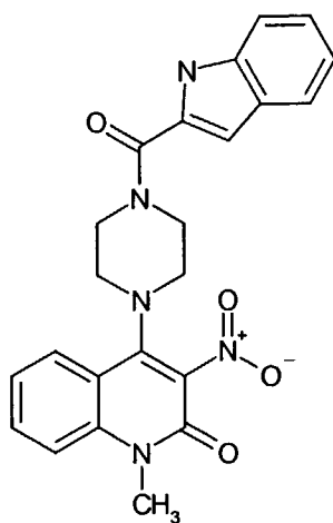
Compound 284
