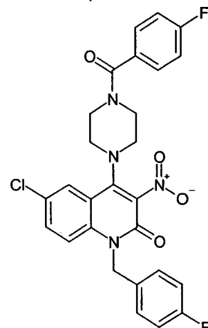
Compound 144
