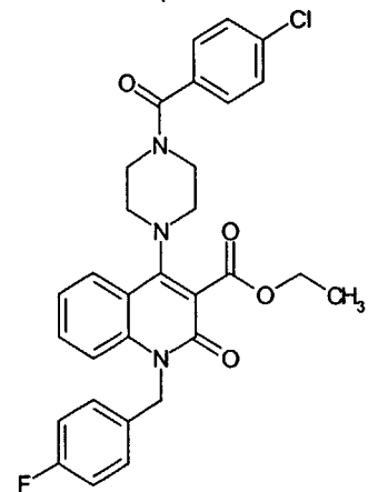
Compound 18
