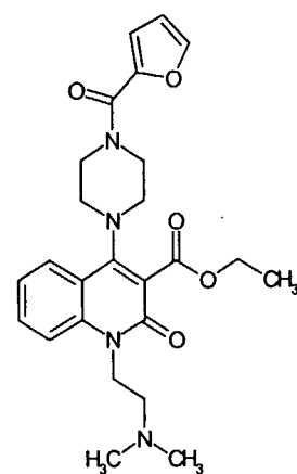
Compound 108
