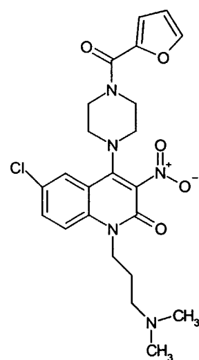
Compound 199
