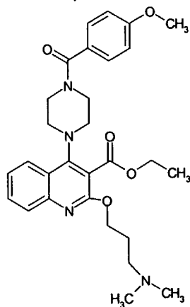
Compound 329
