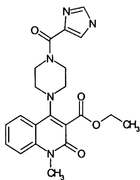
Compound 267
