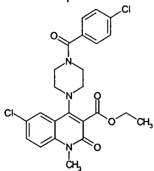
Compound 59
