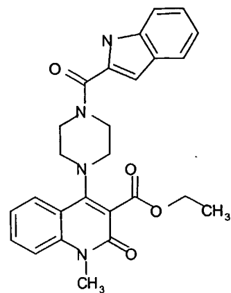
Compound 264
