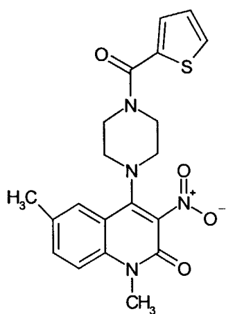
Compound 176
