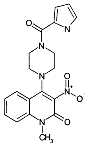
Compound 269
