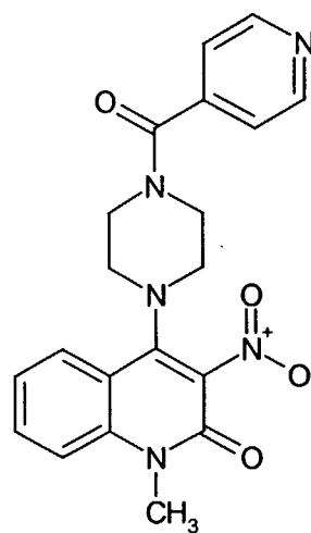
Compound 235
