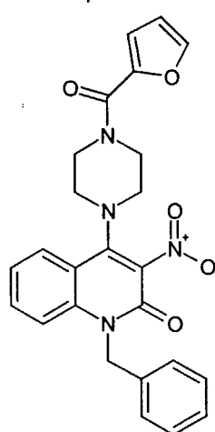
Compound 119
