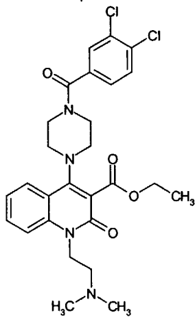
Compound 69
