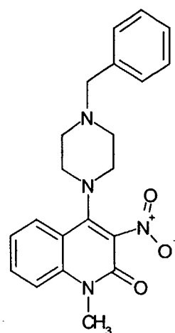
Compound 222
