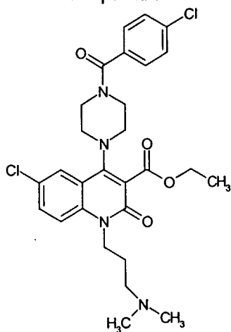
Compound 94
