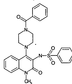
Compound 85
