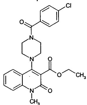
Compound 46
