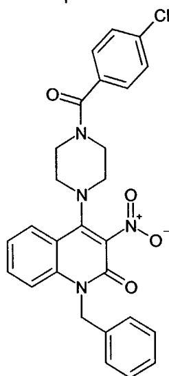
Compound 117
