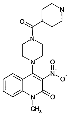
Compound 275
