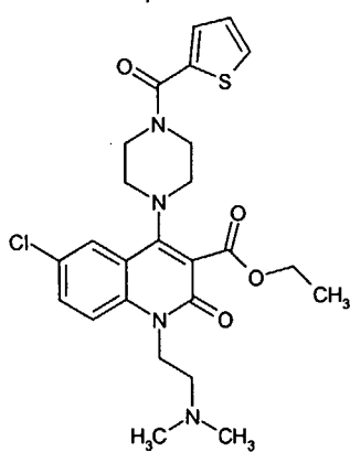
Compound 155
