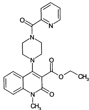
Compound 300
