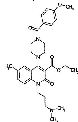
Compound 109
