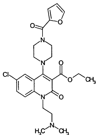
Compound 111
