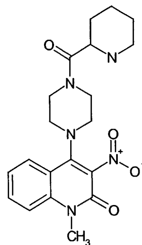
Compound 324
