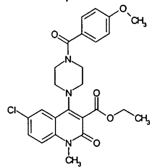
Compound 61
