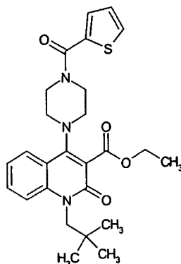
Compound 244
