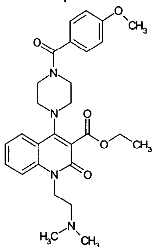
Compound 63
