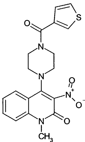
Compound 220
