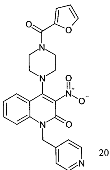
Compound 322
