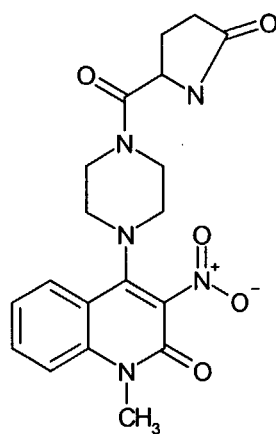
Compound 303
