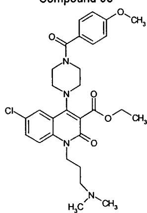
Compound 95
