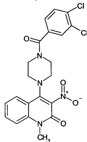
Compound 120
