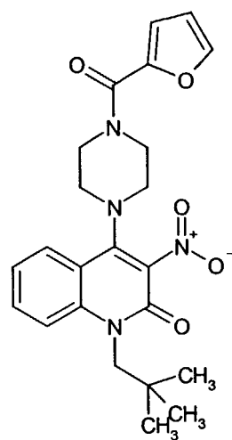
Compound 252
