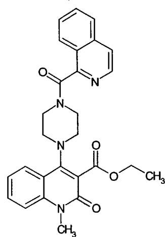
Compound 265
