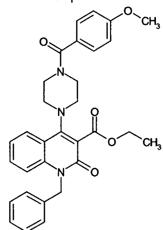
Compound 25
