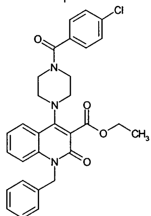
Compound 23
