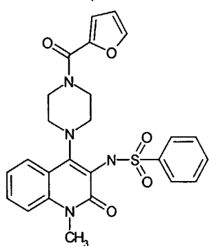
Compound 81
