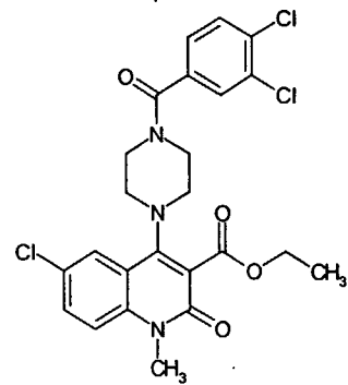
Compound 60
