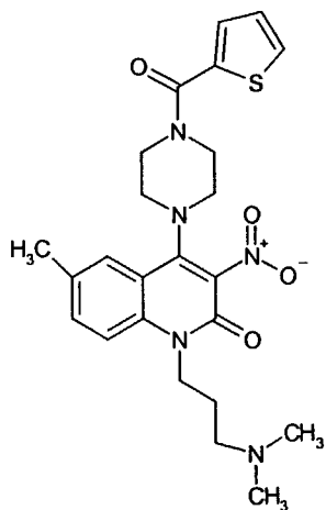
Compound 178
