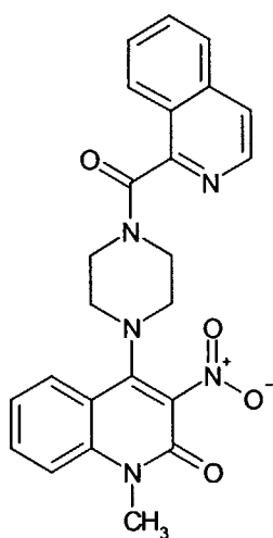
Compound 285
