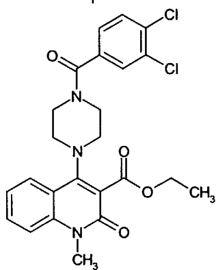
Compound 47
