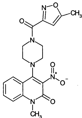
Compound 233
