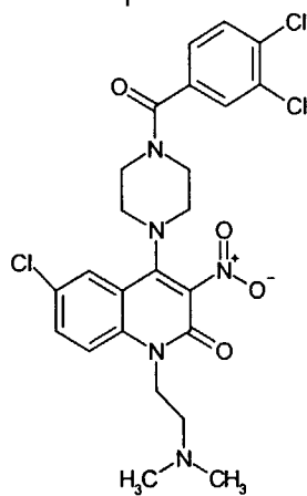
Compound 209
