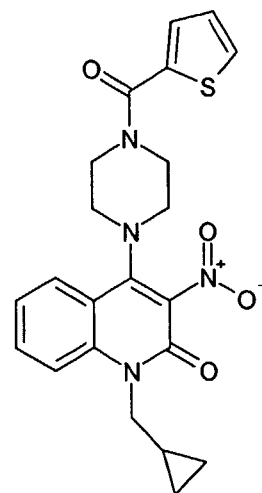
Compound 276
