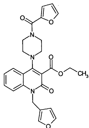
Compound 312
