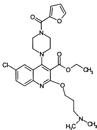
Compound 330
