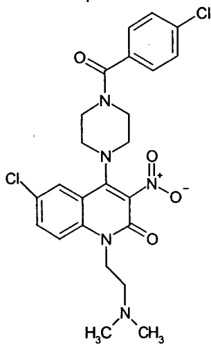
Compound 206
