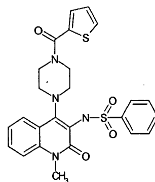
Compound 84
