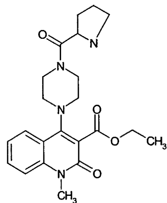
Compound 288
