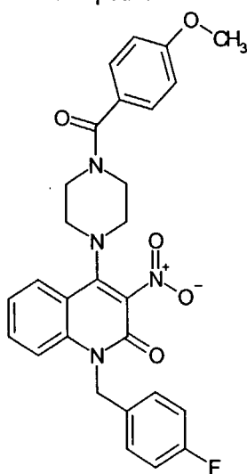
Compound 116
