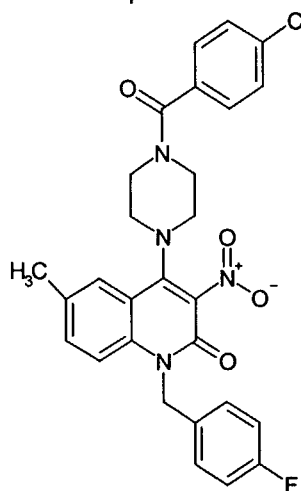
Compound 185
