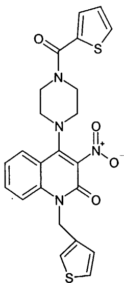
Compound 255
