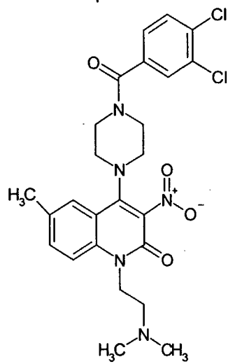
Compound 191
