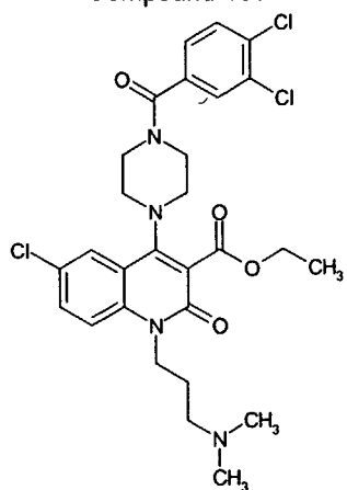
Compound 106
