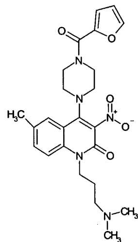
Compound 175
