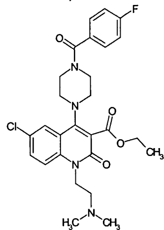
Compound 156
