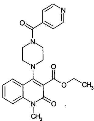
Compound 263
