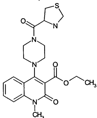
Compound 316
