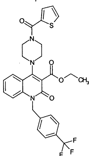
Compound 317
