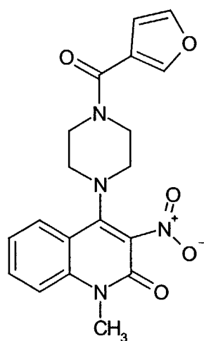
Compound 221
