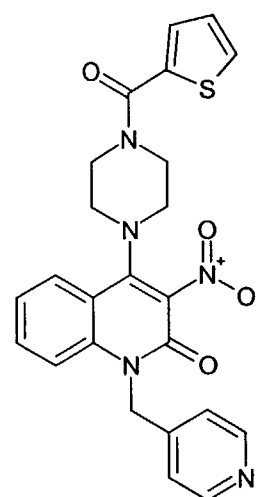
Compound 325
