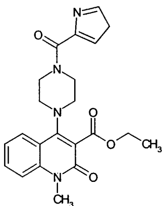
Compound 237
