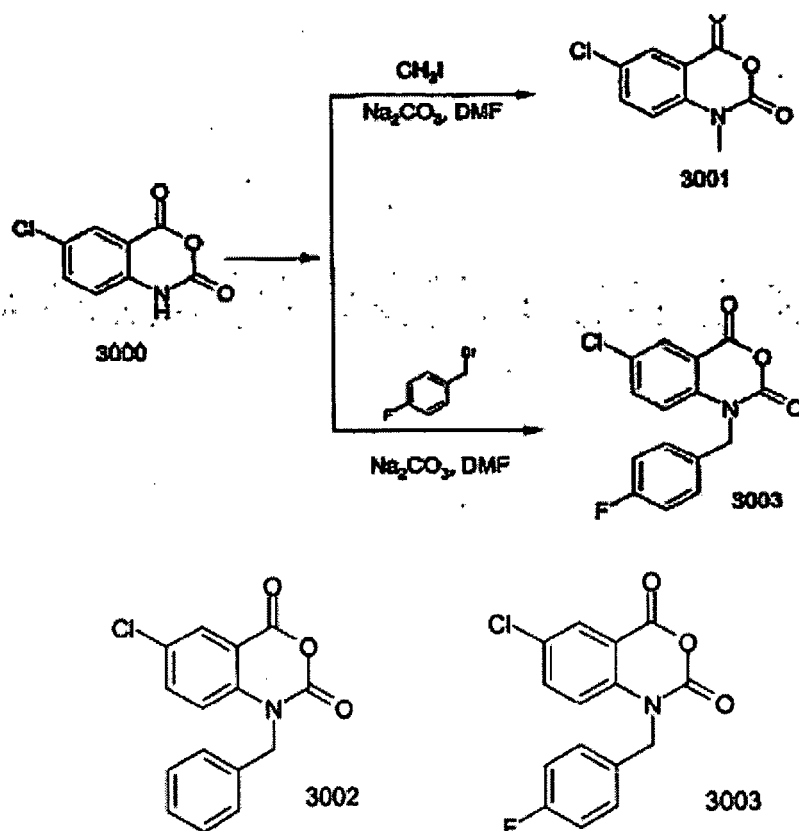
Reaction Scheme 26
