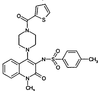
Compound 83
