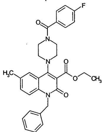
Compound 29
