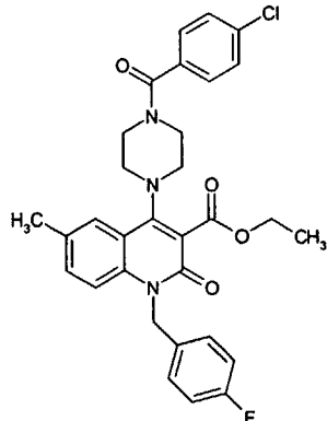
Compound 53
