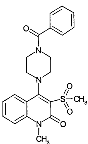
Compound 82
