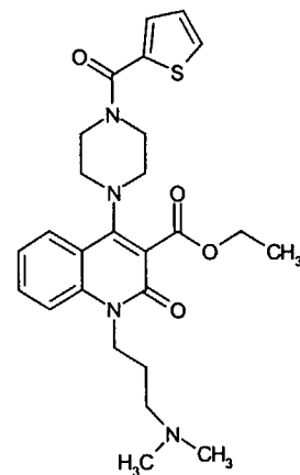
Compound 96
