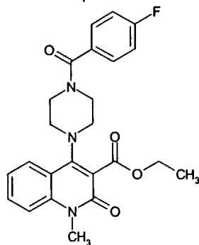
Compound 71
