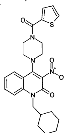
Compound 277
