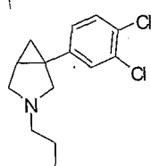
1-(3,4-dichlorophenyl)-3-propyl-3-aza-bicyclo[3.1.0]hexane
