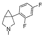
1-(2,4-difluorophenyl)-3-methyl-3-aza-bicyclo[3.1.0]hexane
