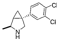
Trans -1-(3,4-dichlorophenyl)-4-methyl-3-aza-bicyclo[3.1.0]hexane
