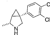
Trans -1-(3,4-dichlorophenyl)-2-methyl-3-aza-bicyclo[3.1.0]hexane
