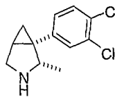
Cis -1-(3,4-dichlorophenyl)-2-methyl-3-aza-bicyclo[3.1.0]hexane
