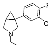
1-(3-chloro-4-fluorophenyl)-3-ethyl-3-aza-bicyclo[3.1.0]hexane
