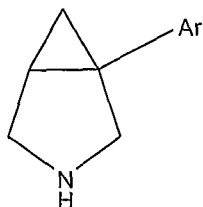
Formula IV
