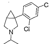
1-(2,4-dichlorophenyl)-3-isopropyl-3-aza-bicyclo[3.1.0]hexane
