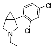
1-(2,4-dichlorophenyl)-3-ethyl-3-aza-bicyclo[3.1.0]hexane
