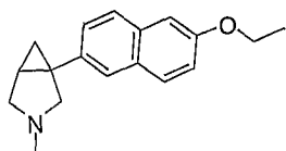
1-(2-ethoxynaphthalen-6-yl)-3-methyl-3-aza-bicyclo[3.1.0]hexane
