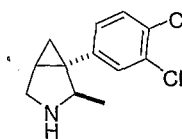
Trans -1-(3,4-dichlorophenyl)-2-methyl-3-aza-bicyclo[3.1.0]hexane
