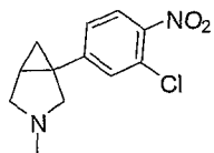
1-(3-chloro-4-nitrophenyl)-3-methyl-3-aza-bicyclo[3.1.0]hexane
