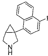
1-(1-fluoronaphthalen-4-yl)-3-aza- bicyclo[3.1.0]hexane
