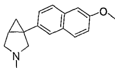
1-(2-methoxynaphthalen-6-yl)-3-methyl-3- aza-bicyclo[3.1.0]hexane
