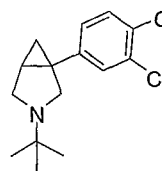
3- tert -butyl-1-(3,4-dichlorophenyl)-3-aza-bicyclo[3.1.0]hexane
