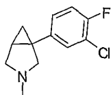
1-(3-chloro-4-fluorophenyl)-3-methyl-3-aza-bicyclo[3.1.0]hexane
