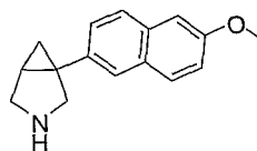
1-(2-methoxynaphthalen-6-yl)-3-aza- bicyclo[3.1.0]hexane
