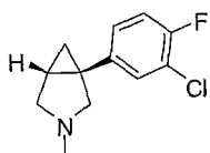
1-(3-chloro-4-fluorophenyl)-3-methyl-3-aza-bicyclo[3.1.0]hexane
