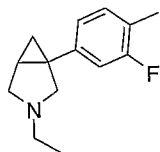
1-(3-fluoro-4-methylphenyl)-3-ethyl-3-aza-bicyclo[3.1.0]hexane
