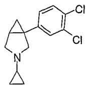
1-(3,4-dichlorophenyl)-3-cyclopropyl-3-aza-bicyclo[3.1.0]hexane
