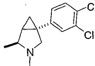
Trans -1-(3,4-dichlorophenyl)-3,4-dimethyl-3-aza-bicyclo[3.1.0]hexane
