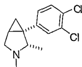
Cis -1-(3,4-dichlorophenyl)-2,3-dimethyl-3-aza-bicyclo[3.1.0]hexane
