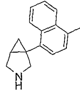
1-(1-fluoronaphthalen-4-yl)-3-aza- bicyclo[3.1.0]hexane
