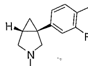
1-(3-fluoro-4-methylphenyl)-3-methyl-3-aza-bicyclo[3.1.0]hexane
