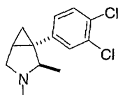
Trans -1-(3,4-dichlorophenyl)-2,3-dimethyl-3-aza-bicyclo[3.1.0]hexane
