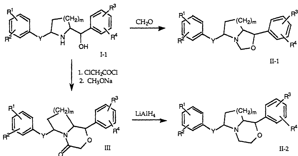
Scheme 2
