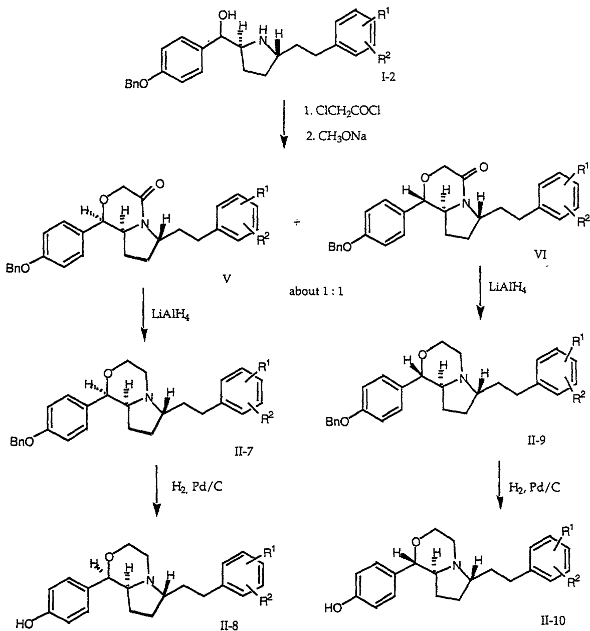
Scheme 4
