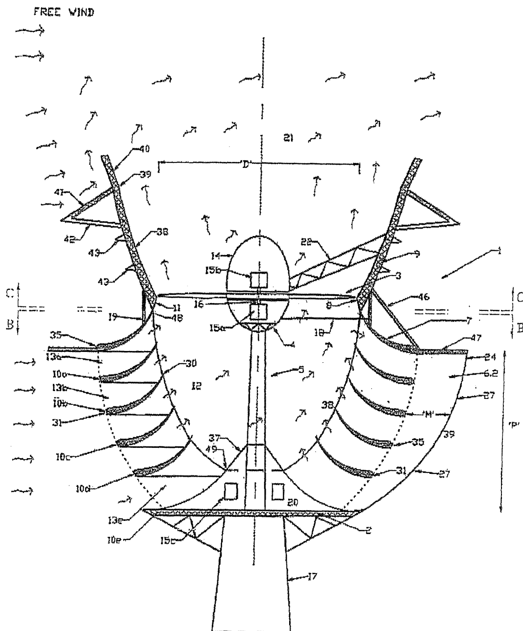
FIG 1: VERTICAL SECTION THROUGH COMPLETE SHROUD ASSEMBLY. AA
