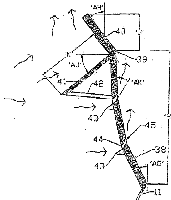
FIG 3: DIFFUSER WALL WITH WEDGE, COLLAR AND BLEED CHANNELS
