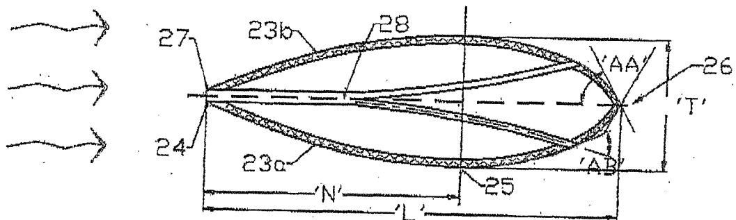
FIG 4: AEROFOIL VERTICAL SUPPORT WALL WITH AIR BLEED CHANNELS
