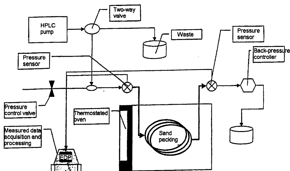
Figure 1 Schematic drawing of the sand packing test setup.
