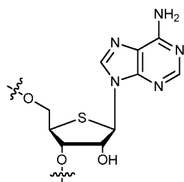
4'Thio-Adenosine
