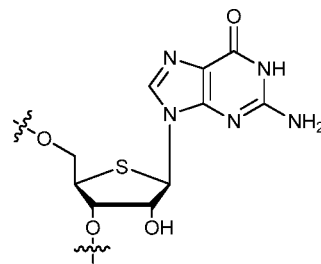
4'Thio-Guanosine
