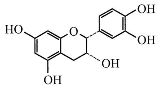
(-) -epicatechin (2R,3R)
