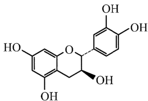
(+) -catechin (2R,3S)
