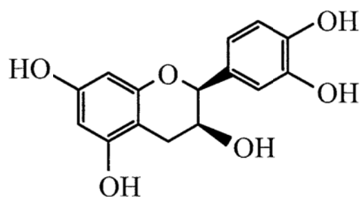
(+) -epicatechin (2S,3S)
