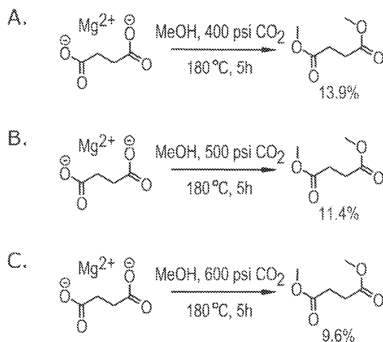
Fig. 6 Pressure Variation
