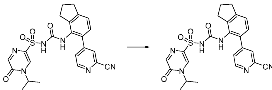
Free acid
