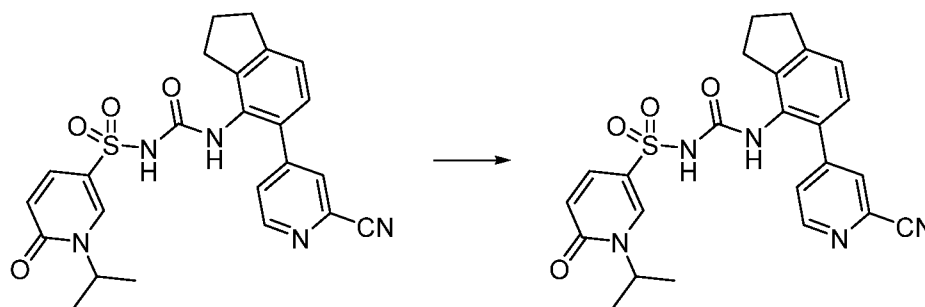
Free acid
