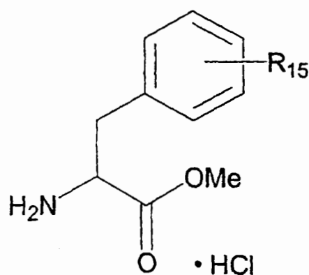
Formula (V);
