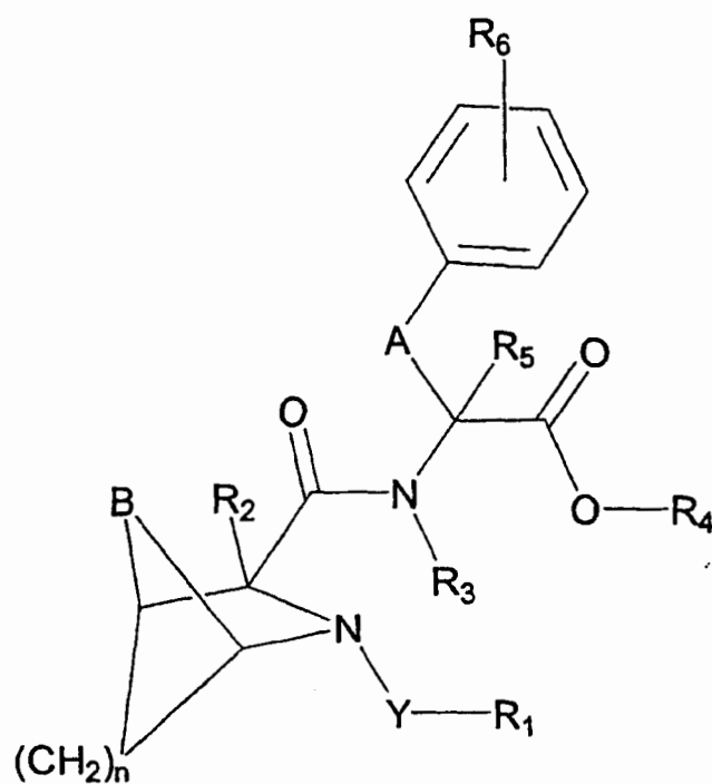
Formula (II)
