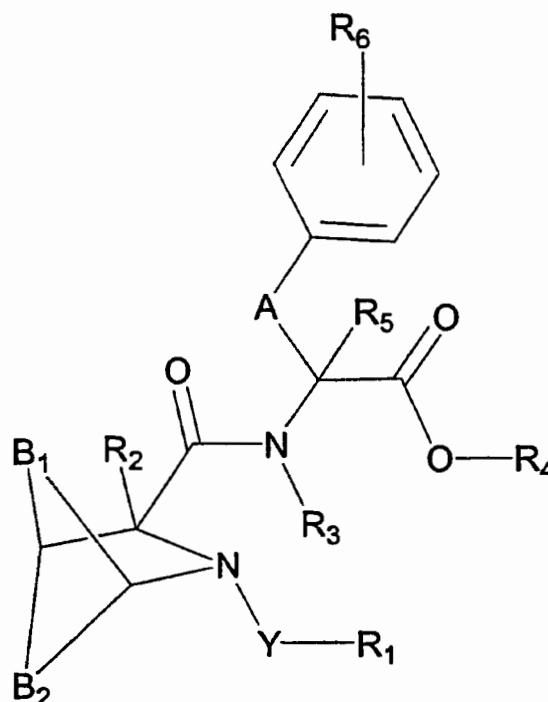
Formula (I)
