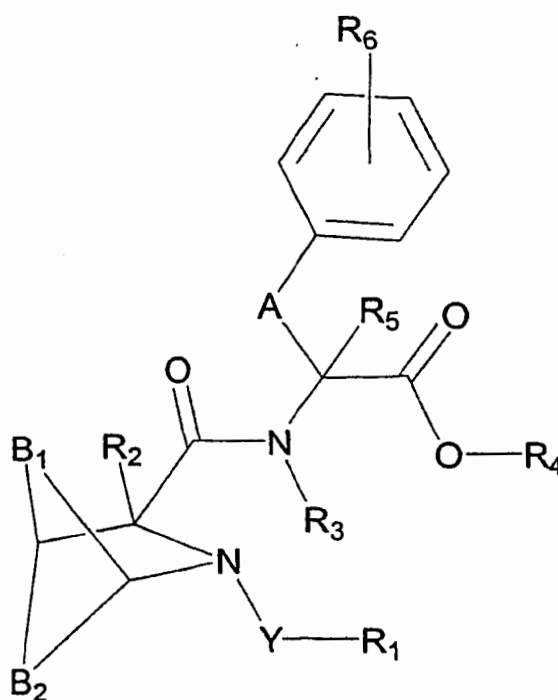
Formula (I)
