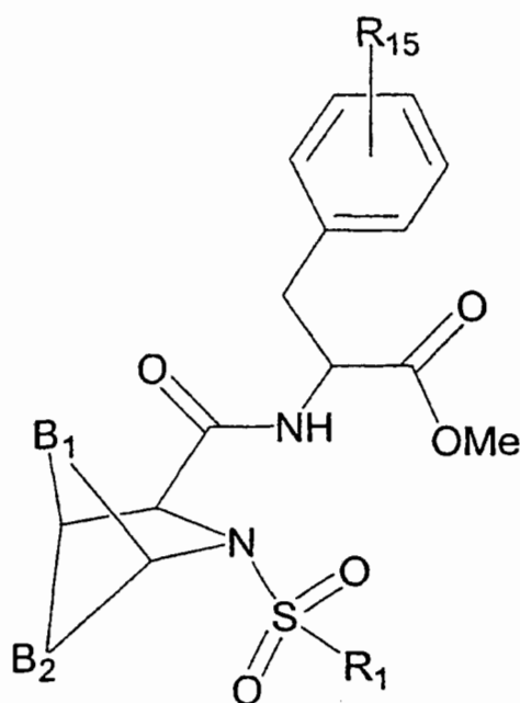
Formula (III)
