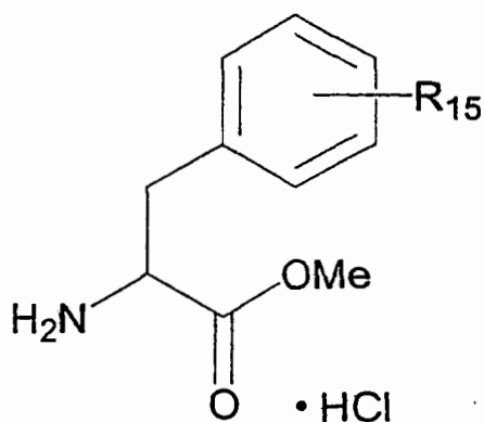
Formula (V);
