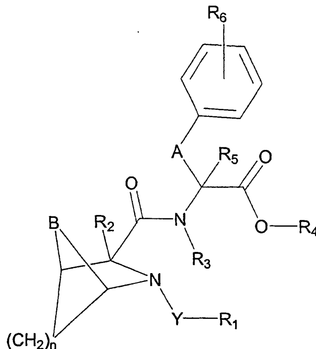
Formula (II)
