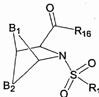
Formula (IV)
