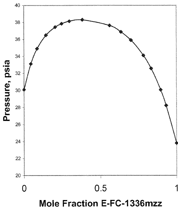
FIGURE 6. E-FC-1336mzz and n-Butane at 20 C
