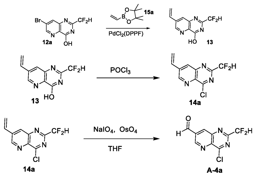
Scheme 5
