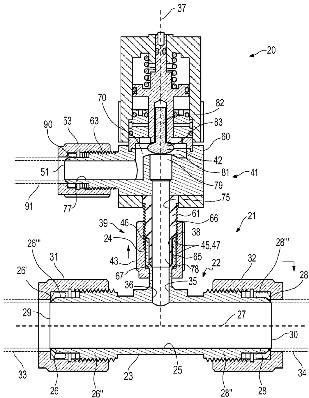
SECTION 5-5
