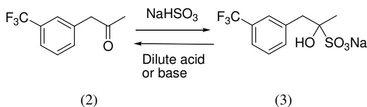
Scheme 3: Purification of ketone (2) via formation of a ketone bisulfite adduct (3).
