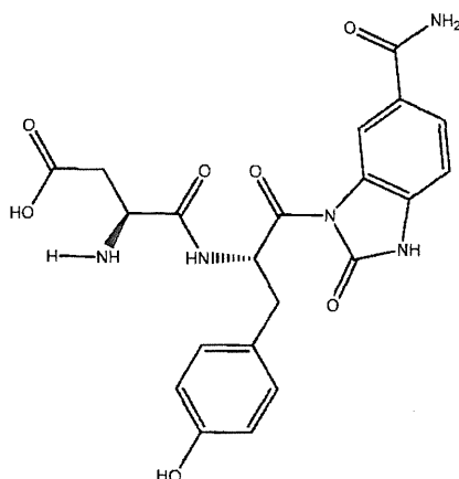
Acylurea-activated DY Dipeptide
