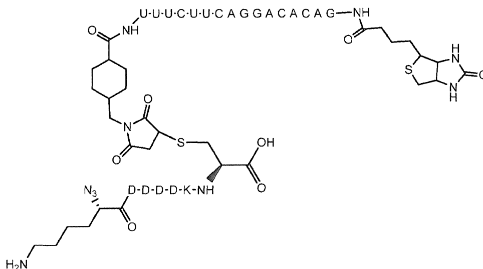
Templated Assembly Reactant 4B
