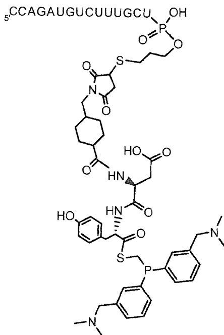
Templated Assembly Reactant 4A
