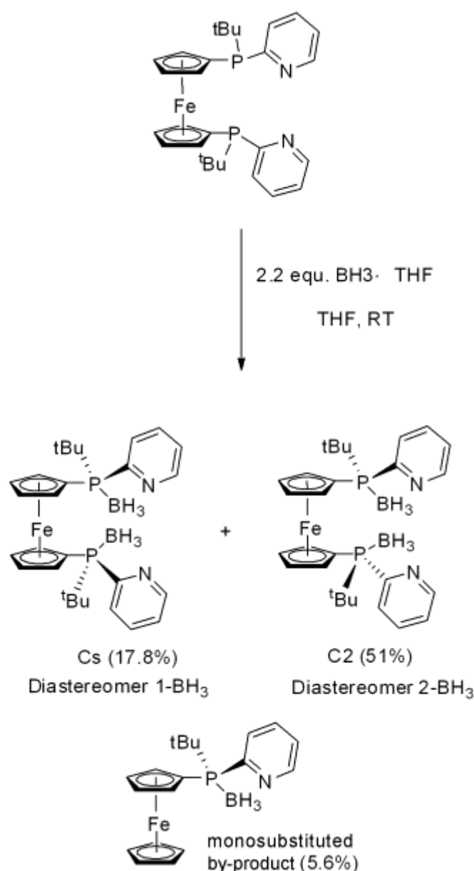
Scheme 2: Synthesis of the borane adducts; Cs: mirror symmetry based on the plane through the Fe atom at right angles to the molecule axis; C 2 : twofold symmetry based on the rotation about the Fe atom
