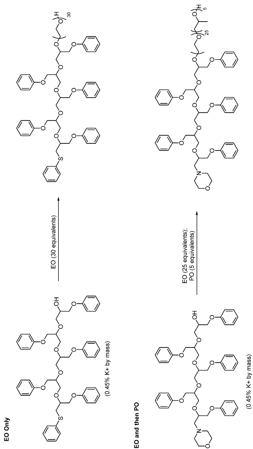
Scheme 3. Alkoxylation Reactions:
