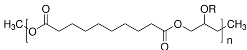
Poly(glycerol sebacate)
