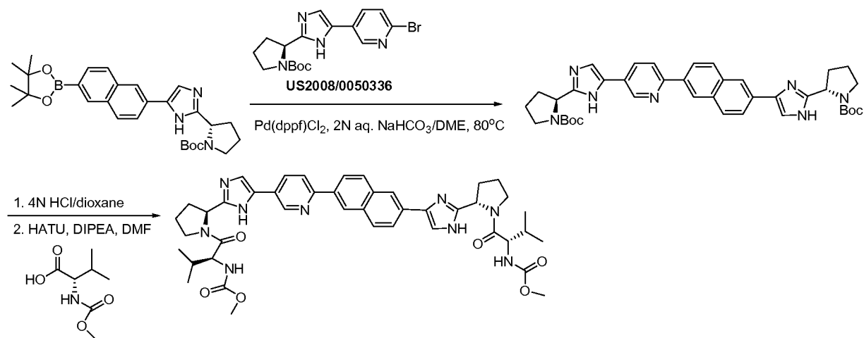
Scheme 12-7
