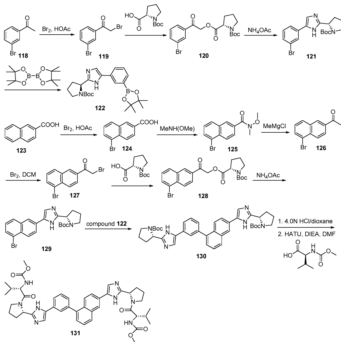
Scheme 8-1
