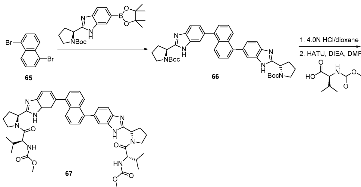
Scheme 5-1
