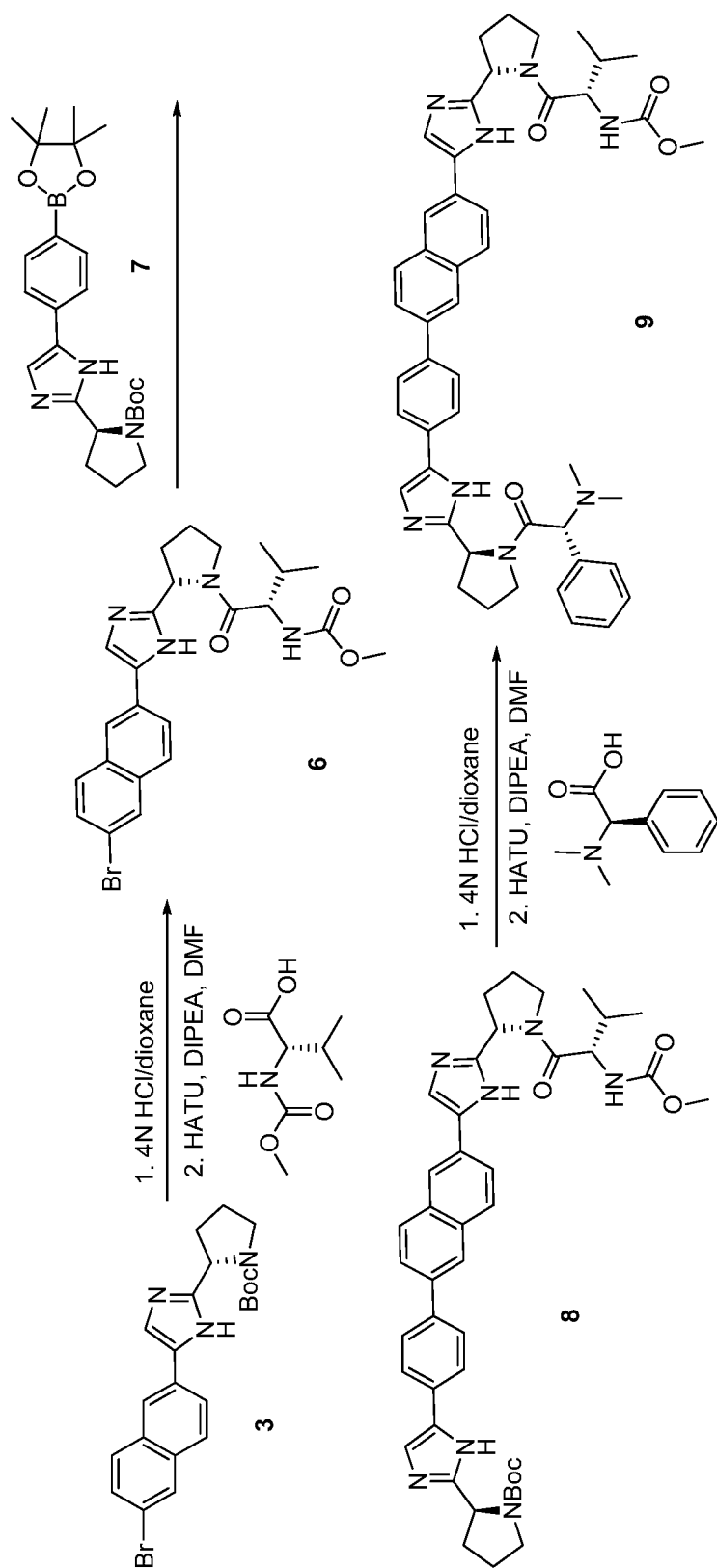
Scheme 1-2
