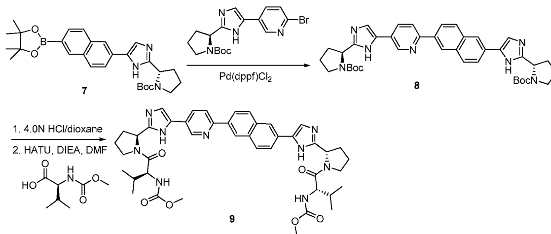
Scheme 3-2
