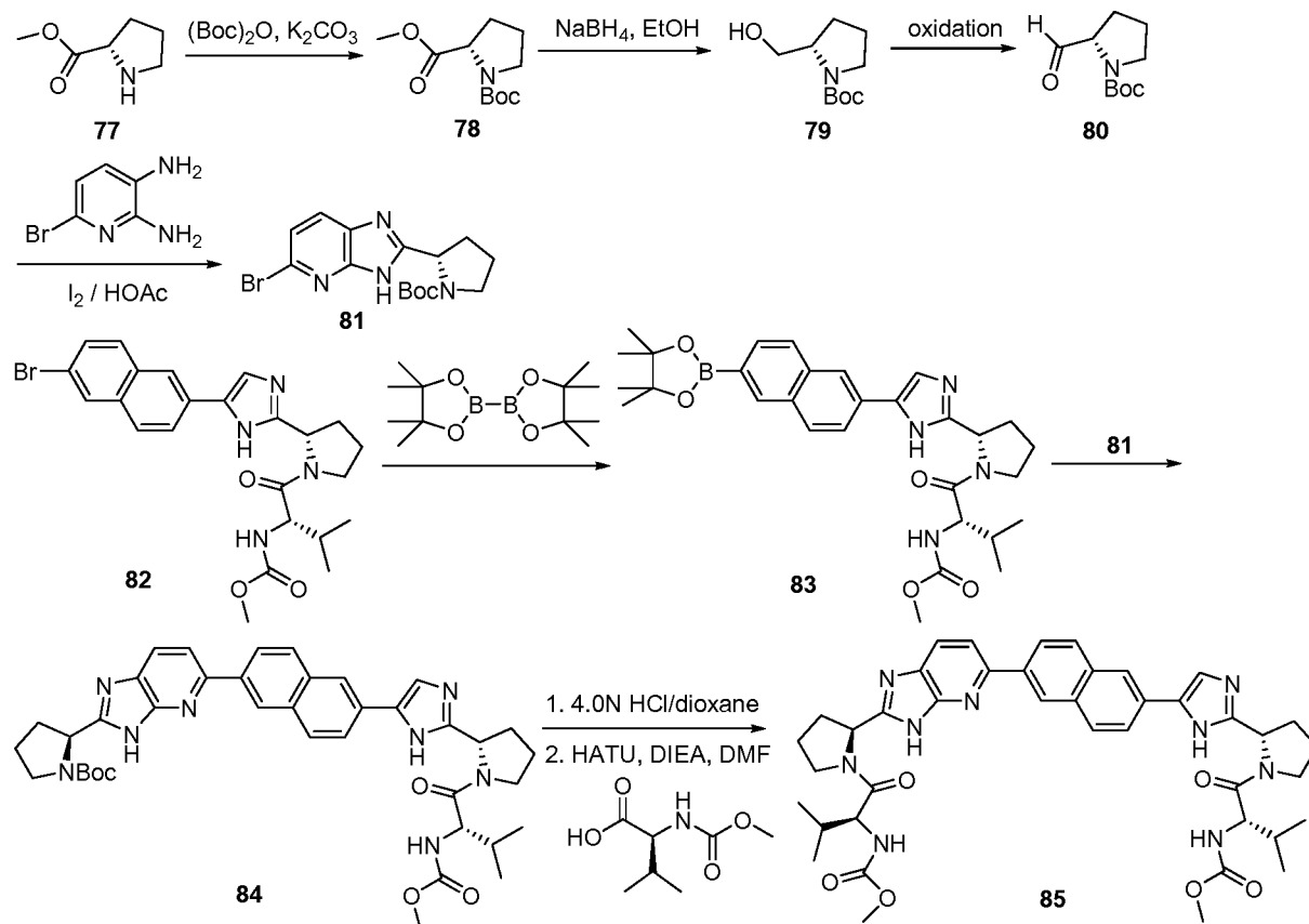
Scheme 6-2
