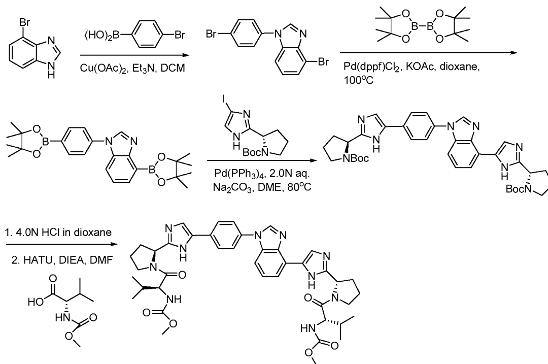
Scheme 12-4
