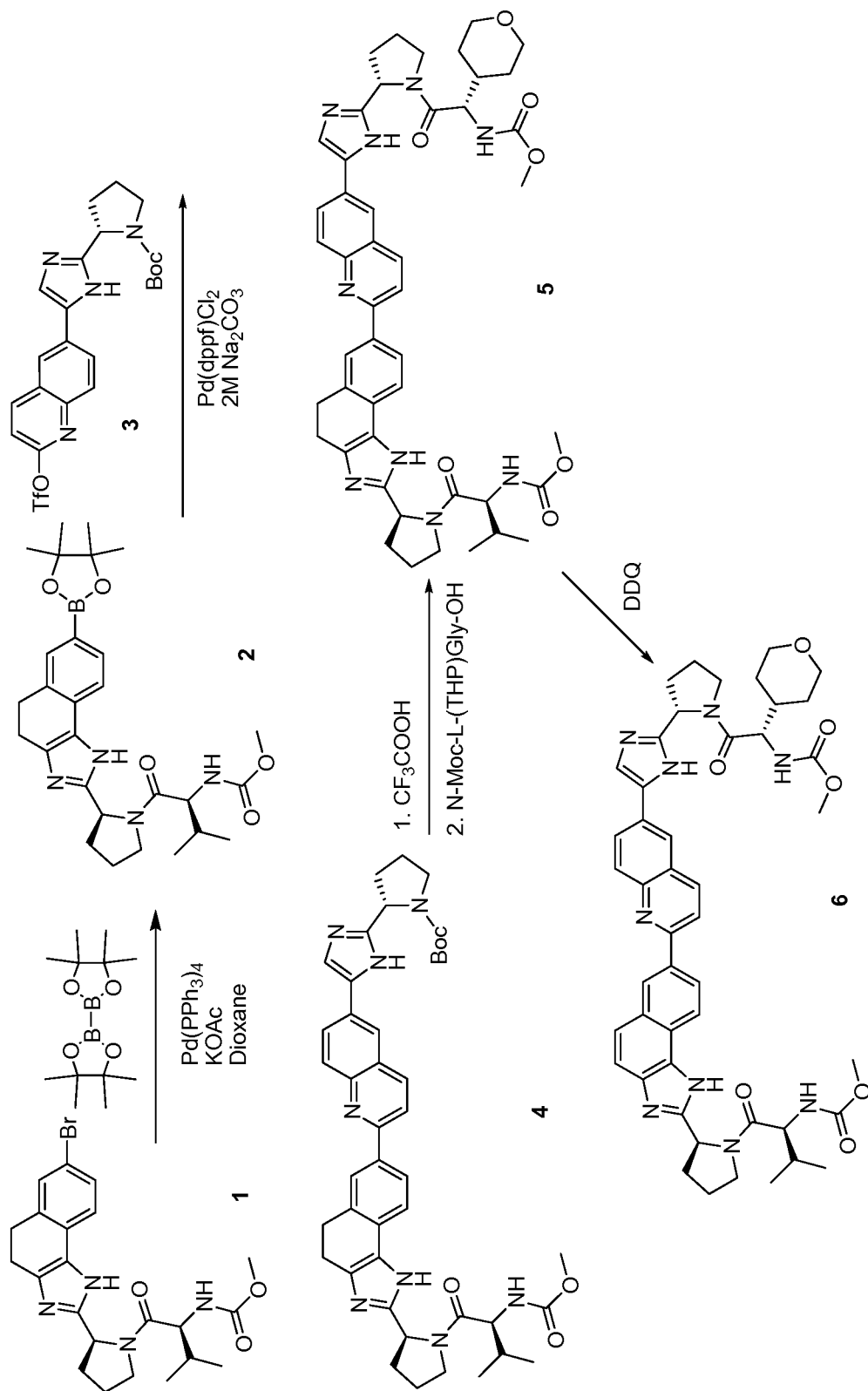
Scheme 11-1
