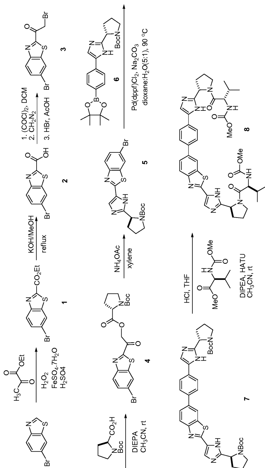
Scheme 12-9
