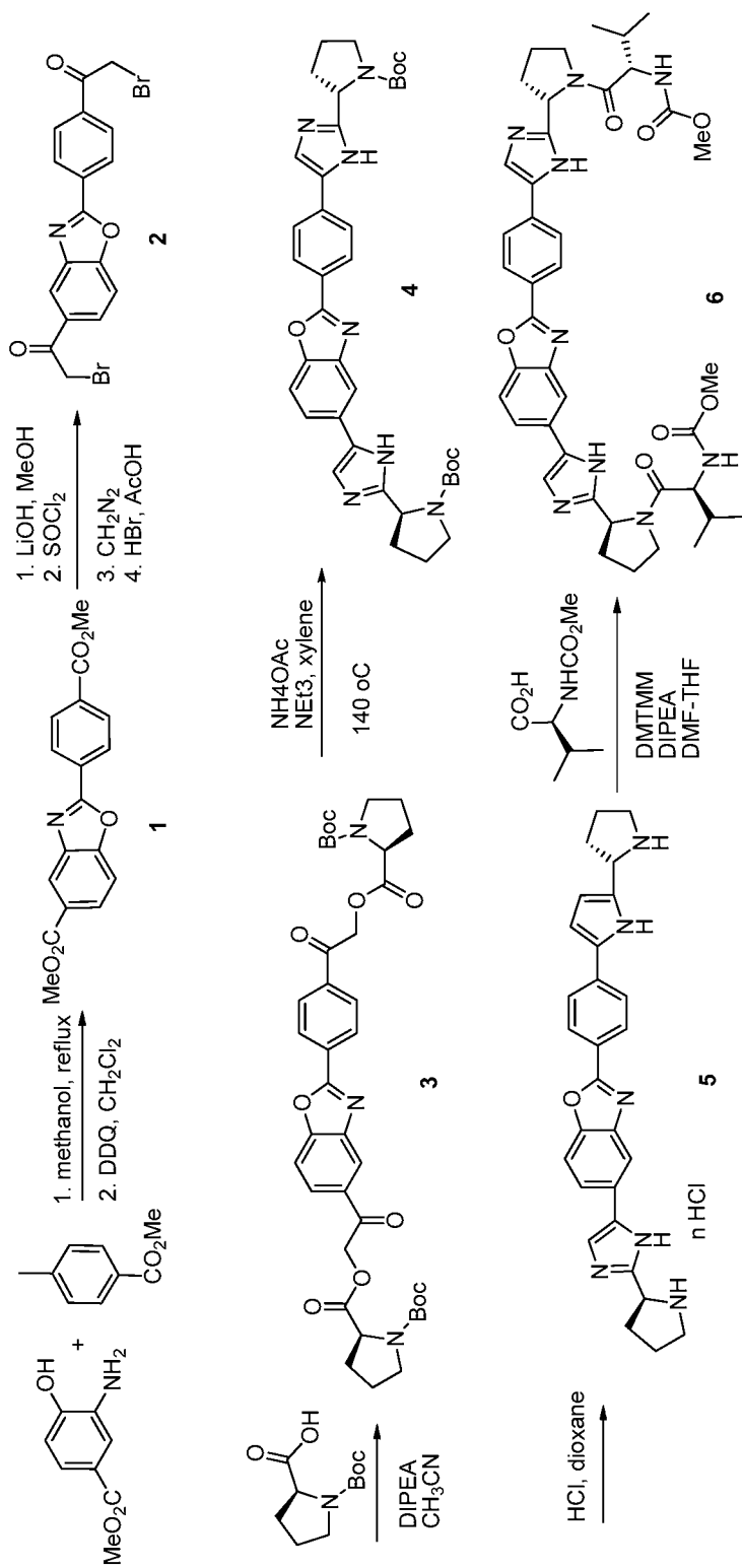
Scheme 9-3
