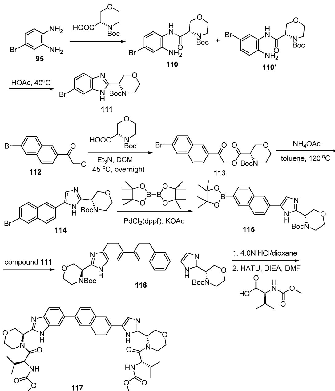
Scheme 6-4
