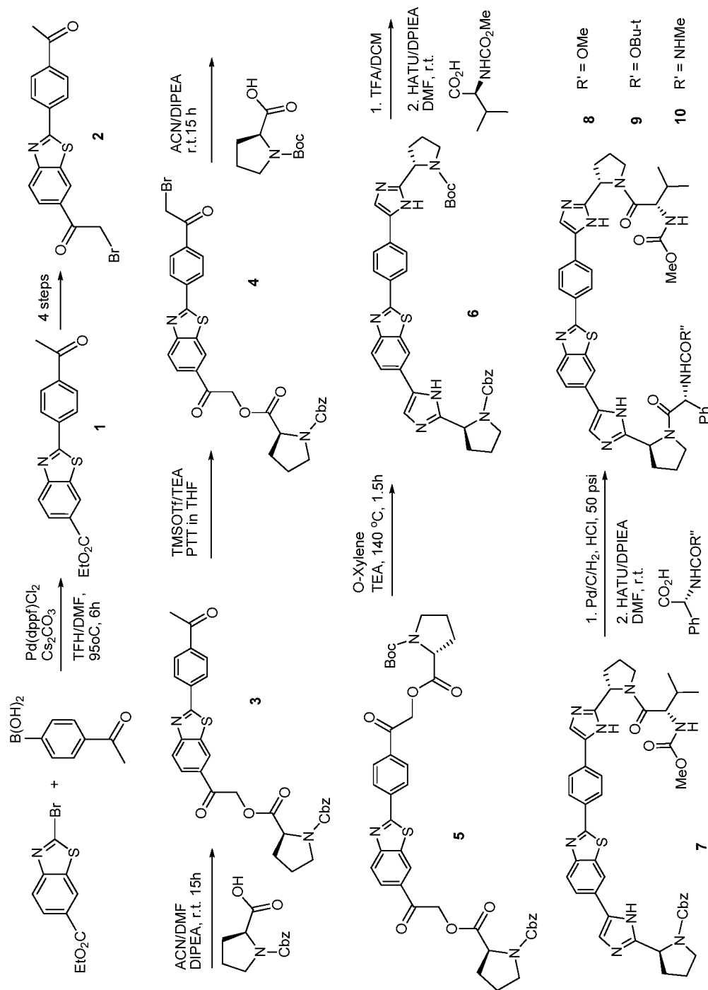
Scheme 9-4
