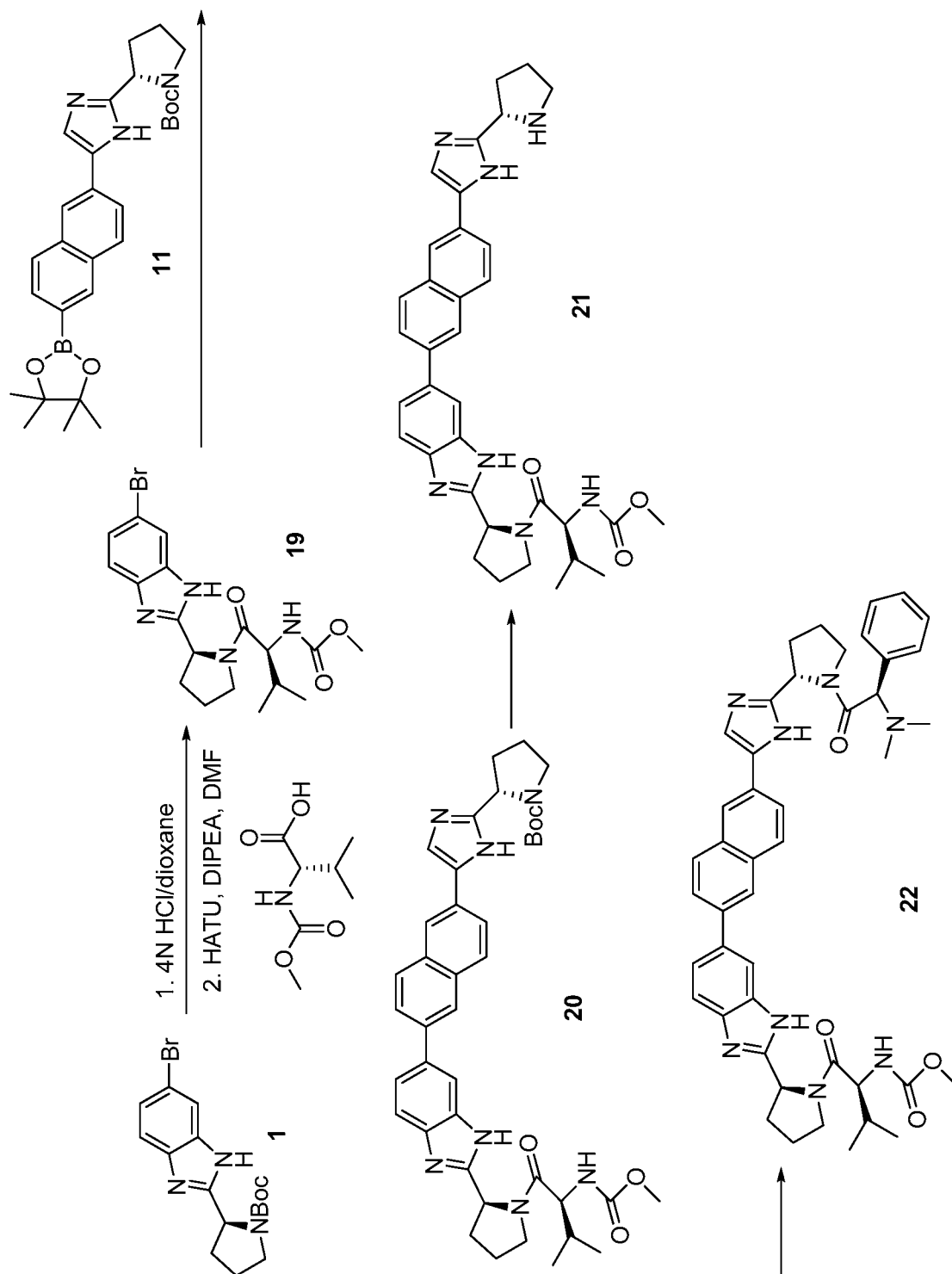
Scheme 2-3
