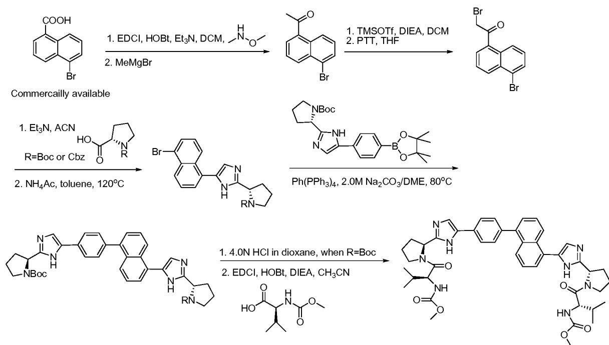
Scheme 12-6
