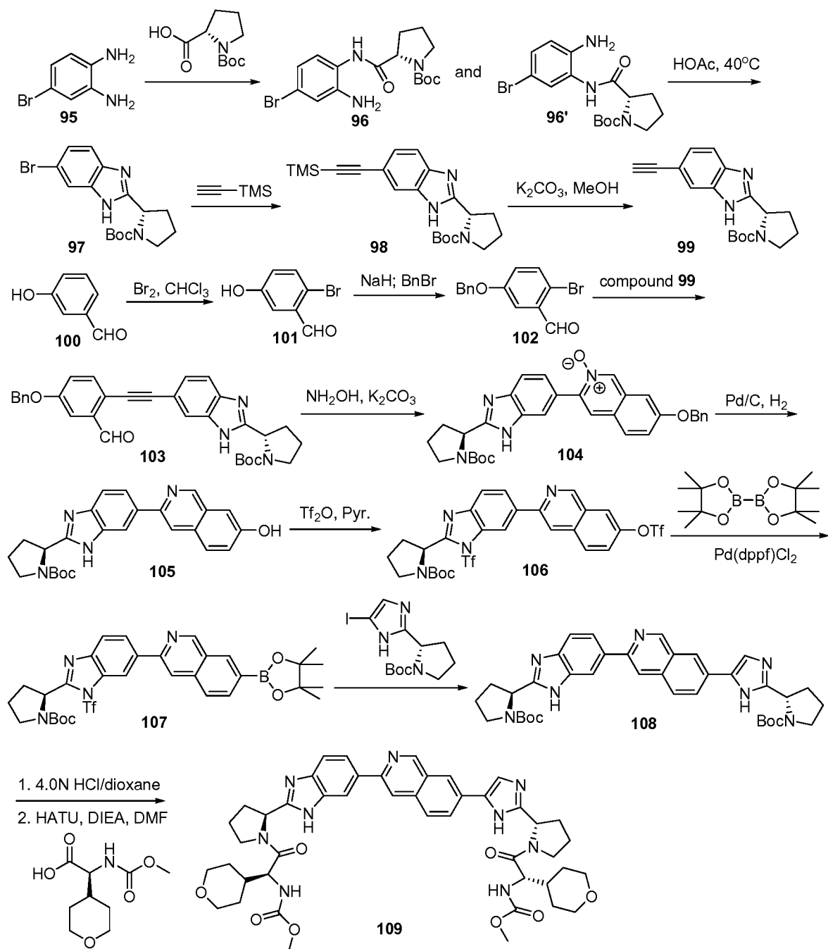
Scheme 6-3
