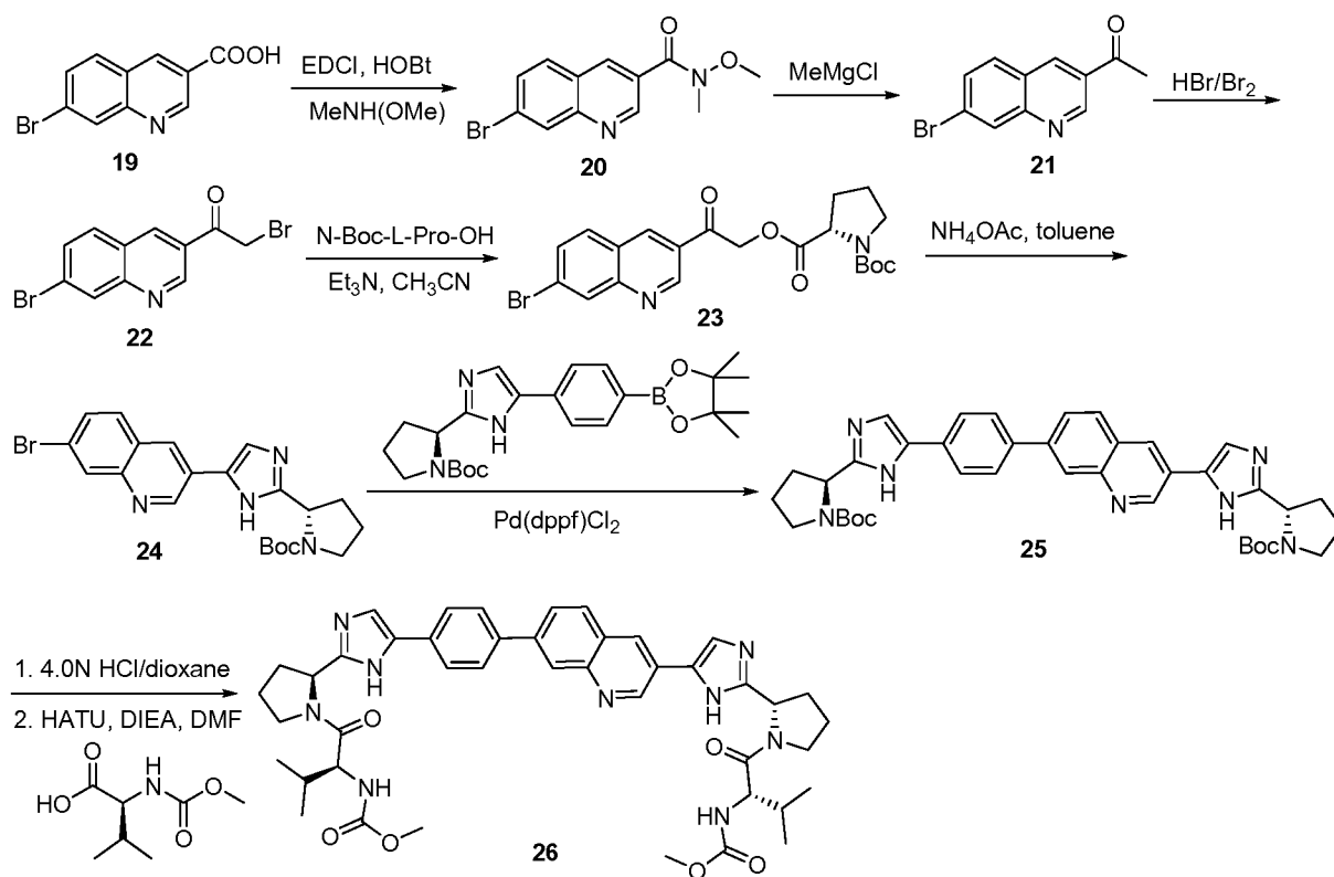
Scheme 3-4
