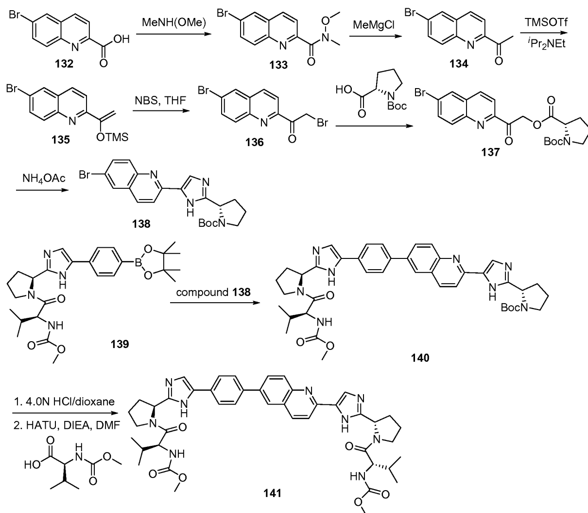
Scheme 3-8
