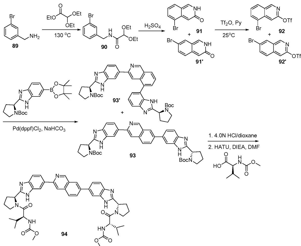
Scheme 7-2
