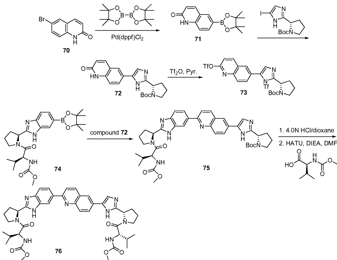
Scheme 6-1
