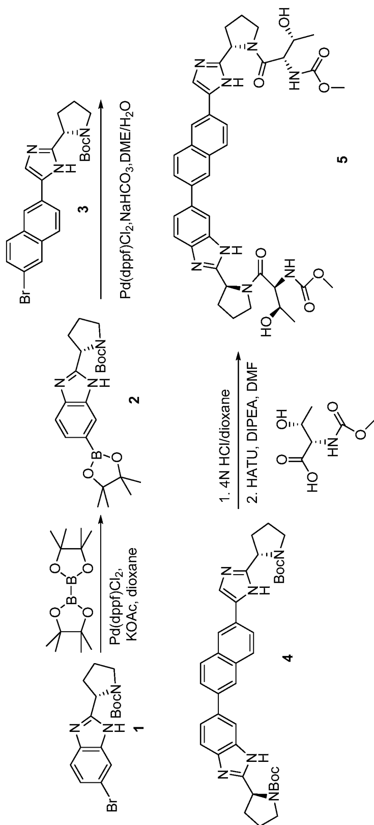
Scheme 2-1
