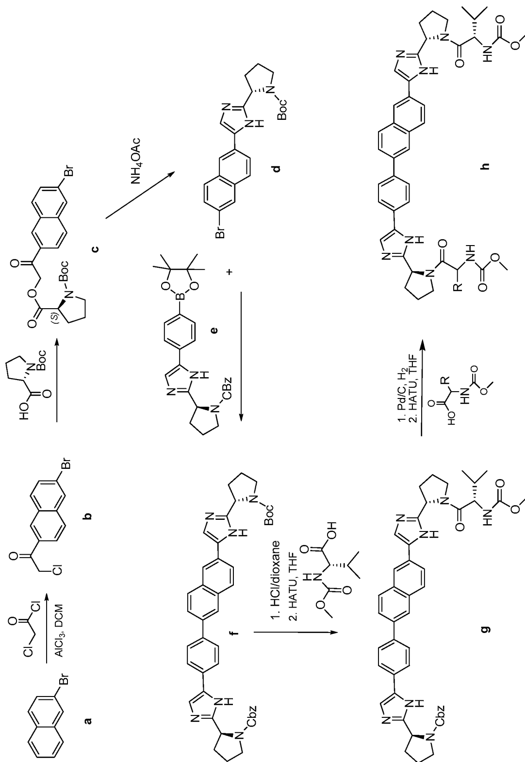
Scheme 1-1
