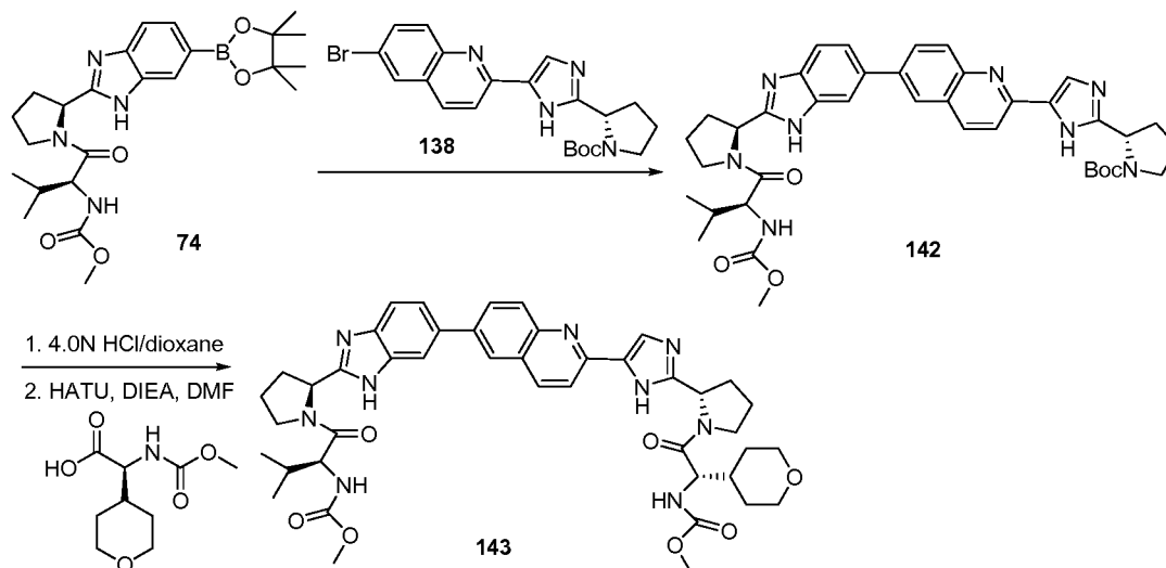
Scheme 2-4
