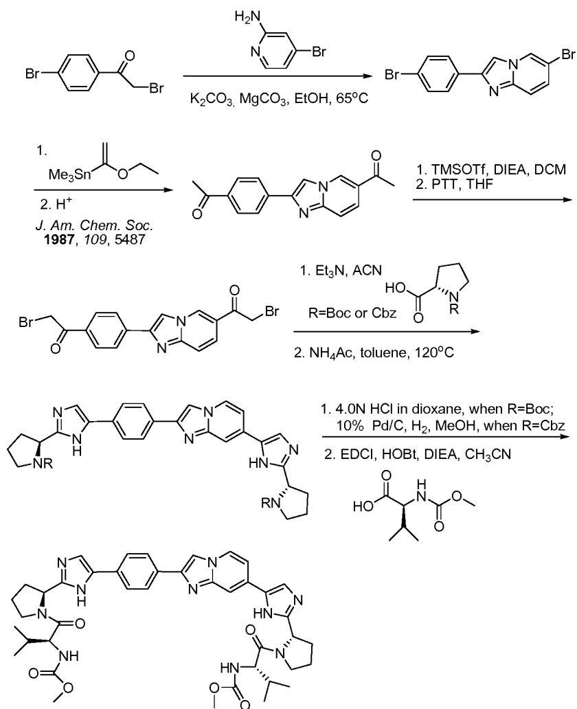
Scheme 12-5
