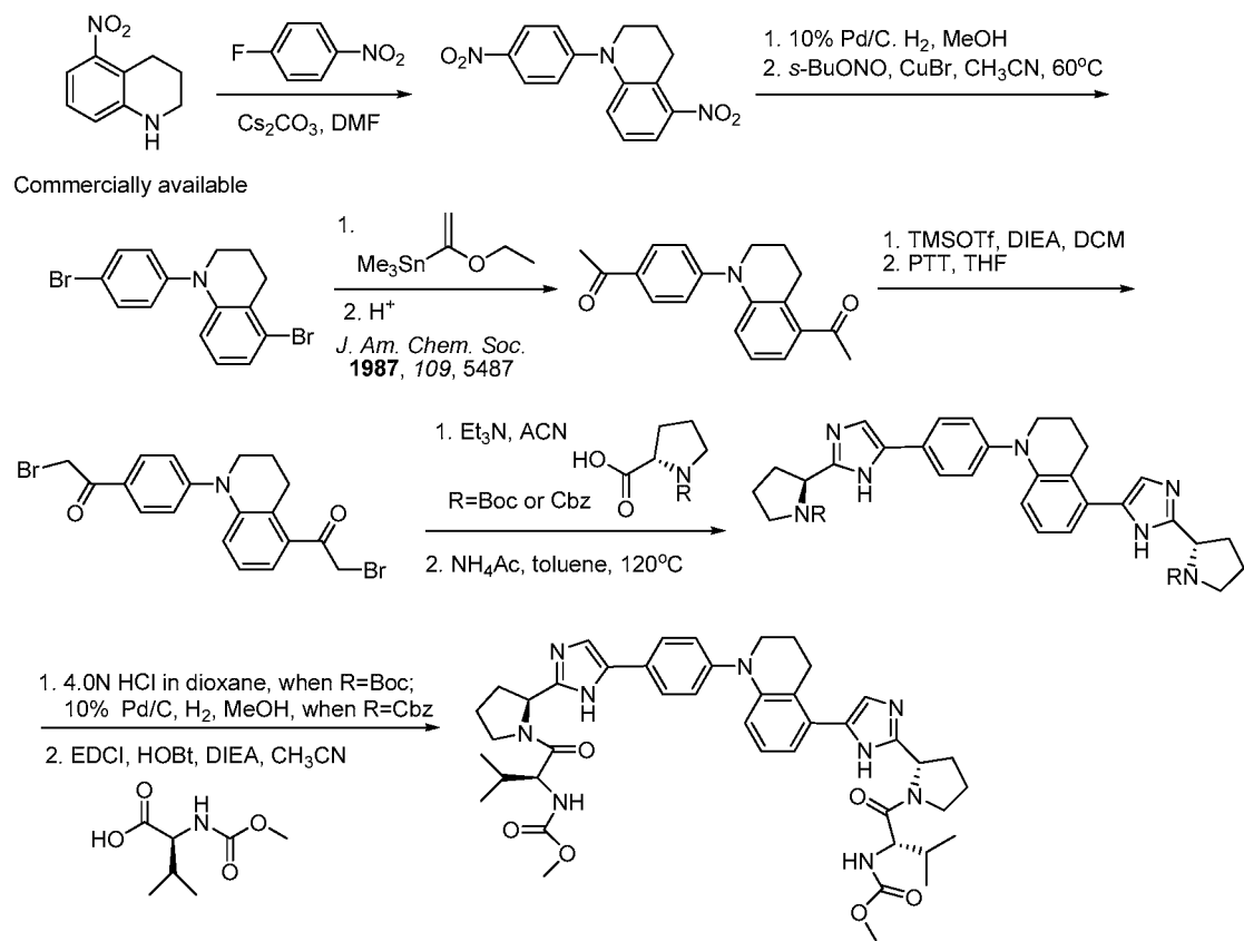
Scheme 12-3
