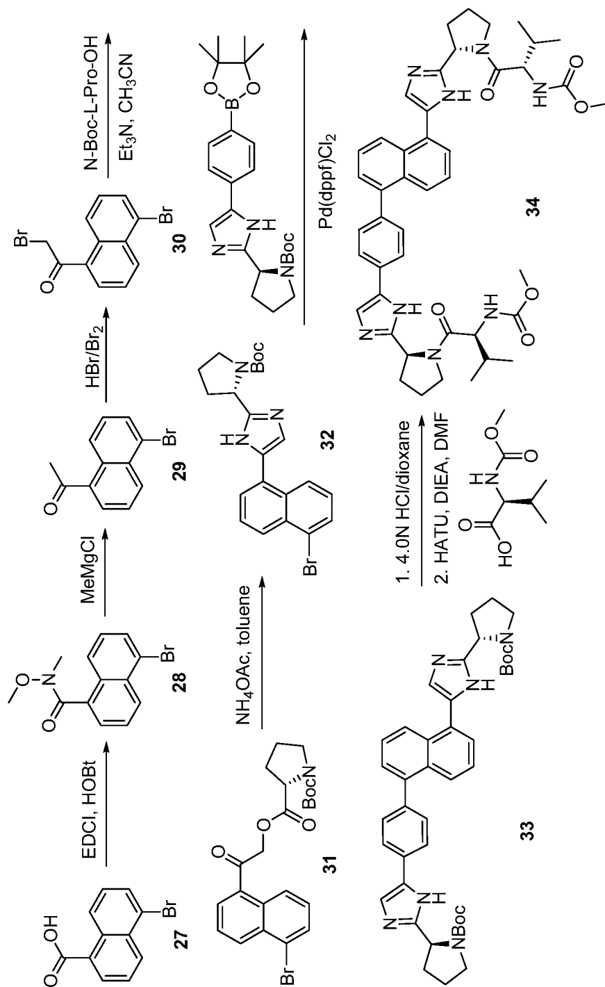
Scheme 4-1
