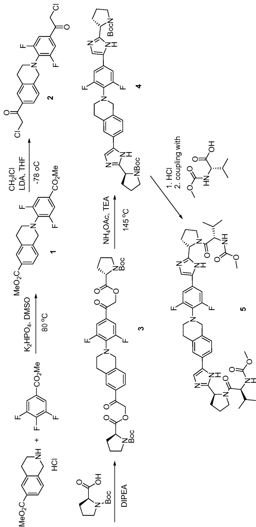
Scheme 10-1
