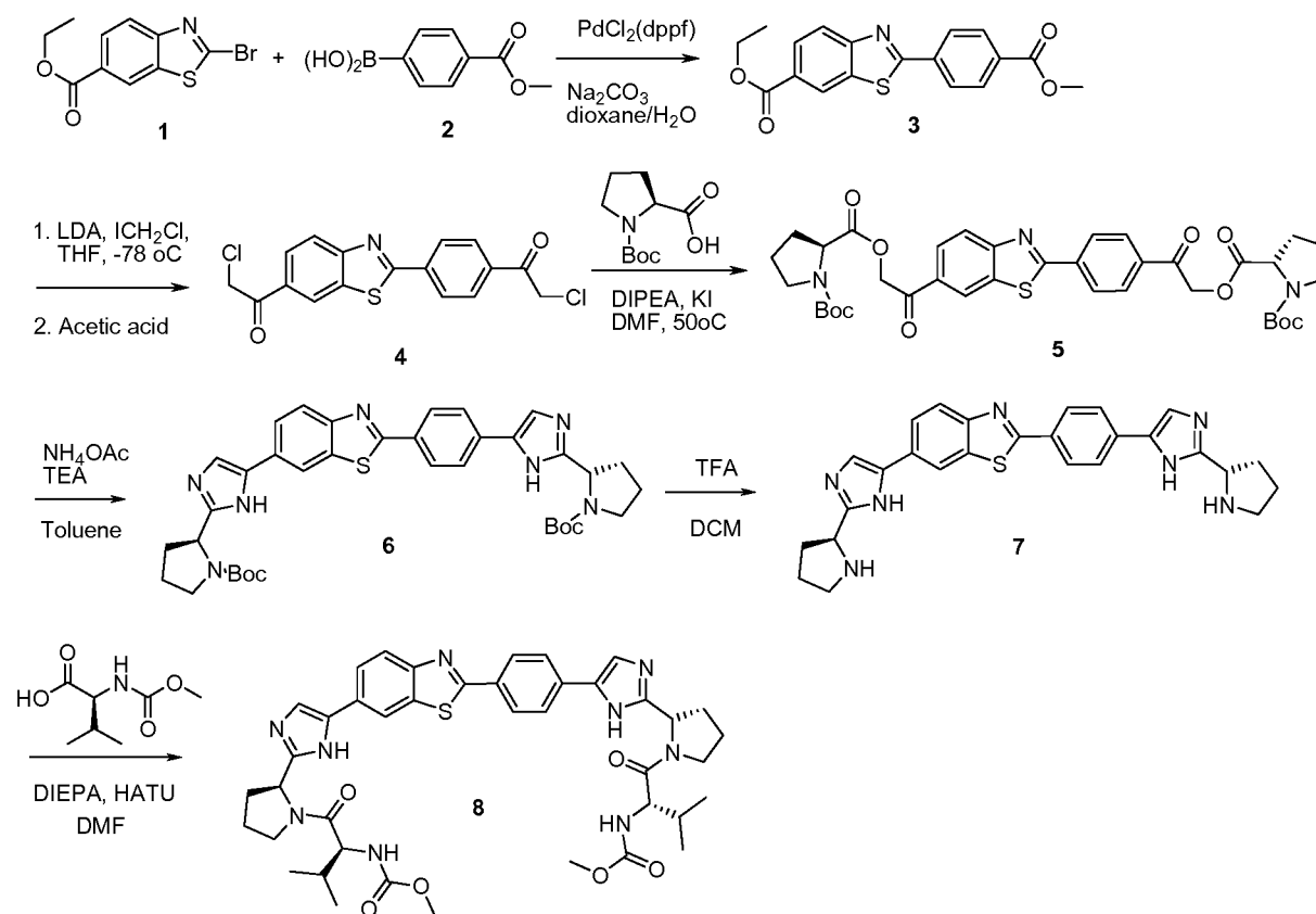
Scheme 9-1
