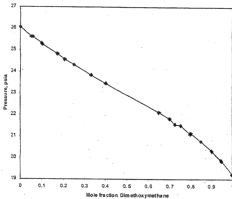
FIGURE 7. Z-FC-1336mzz and Dimethoxymethane at 49.99 C
