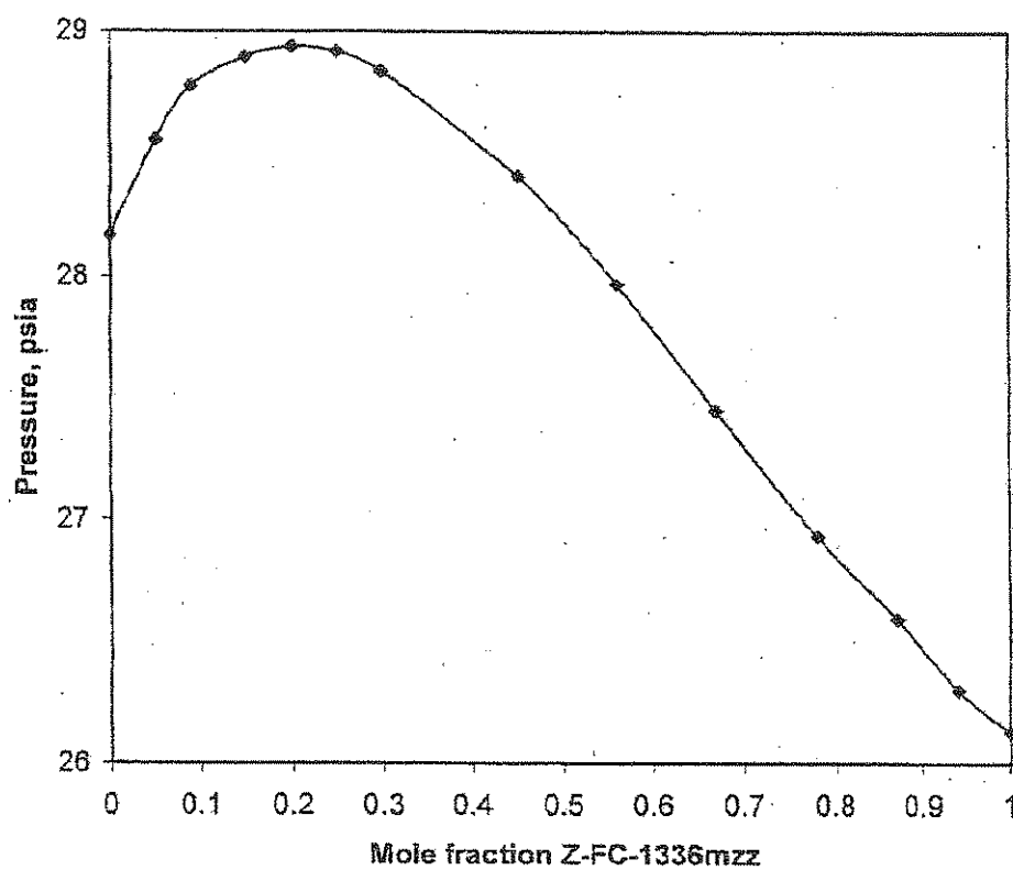
FIGURE 1. VLE DATA for Z-FC-1336mzz/Methyl Formate at 50.1 C
