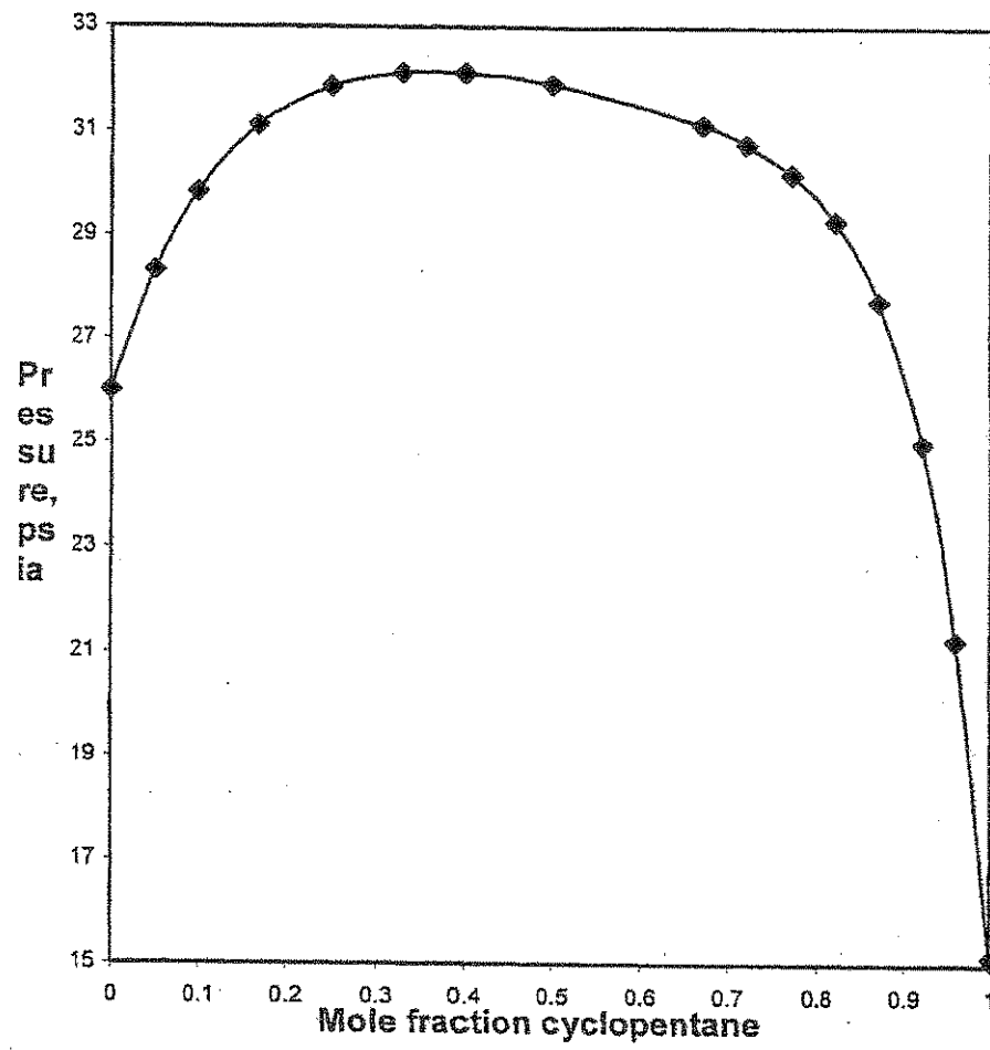
FIG. 8 - Z-FC-1336mzz and Cyclopentane at 50 C
