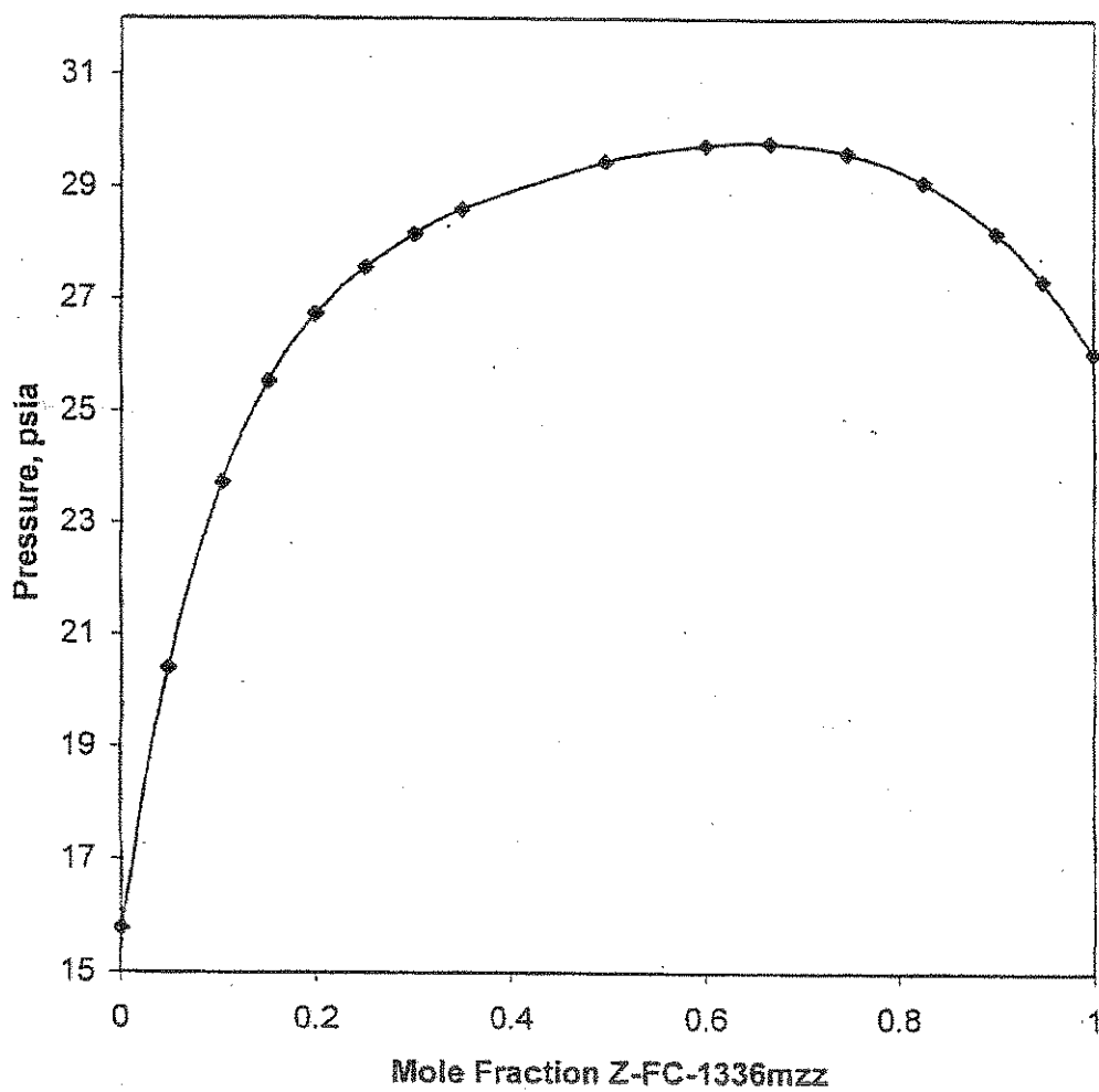
FIGURE 5. Z-FC-1336mzz and trans-1,2-Dichloroethylene at 50.07 C
