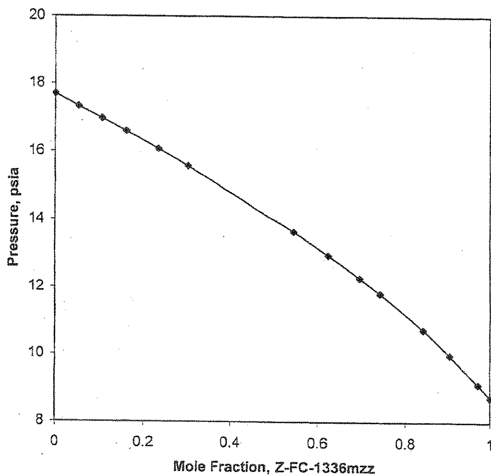
Figure 6. Z-FC-1336mzz and HFC-245fa at 20 C
