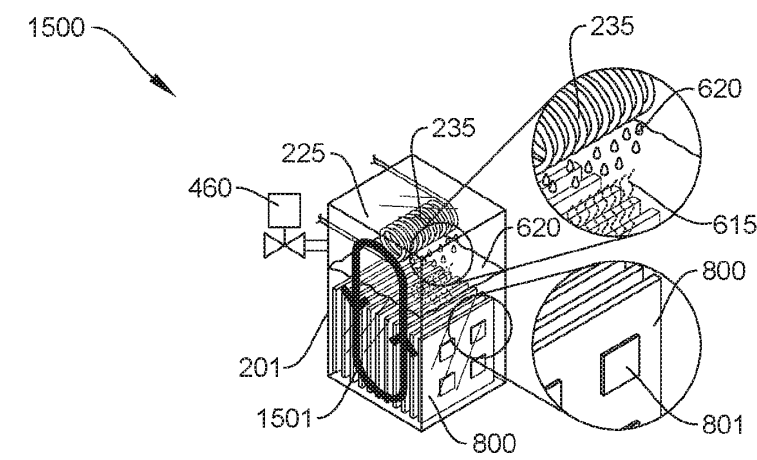
FIG. 15 (PRIOR ART)
