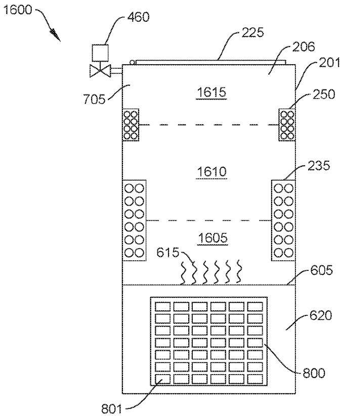
FIG. 16 (PRIOR ART)
