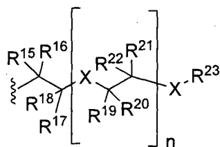
Formula (IIb)
