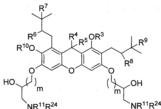
Formula (III)
