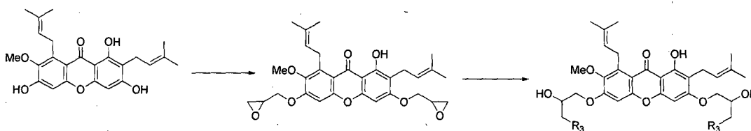
Scheme 1-3
