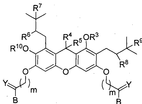
Formula (II)
