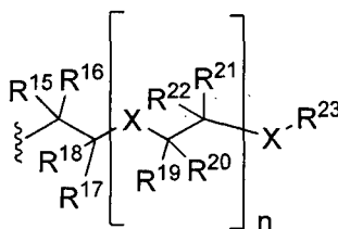
Formula (IIIb)
