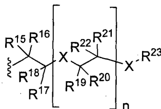
Formula (Ib)
