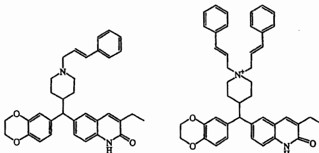
compound 14
