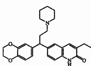
compound 16
