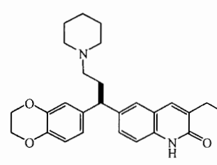
Compound 145
