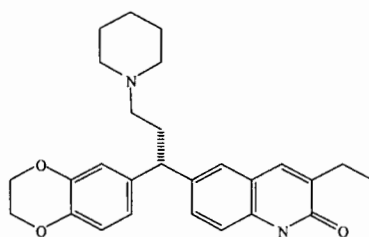
Compound 144
