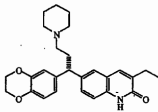
Compound 144
