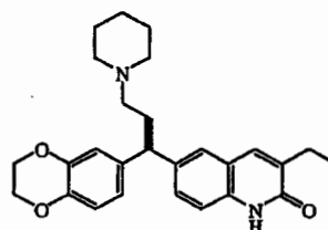
Compound 145
