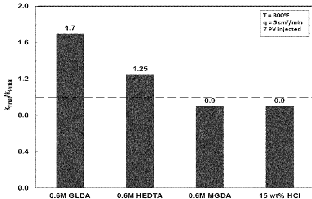
Fig. 3 - Permeability ratio for the Berea sandstone cores treated with 15 wt% HCl and 0.6M chelating agent (pH =4) at 300°F and 5 cm³/min.
