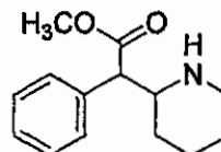
Methylphenidate
