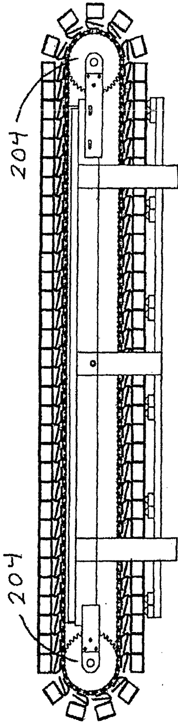
SECTION B-B
