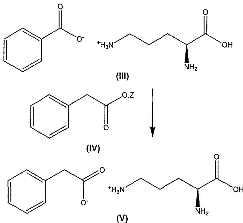
Scheme 2
