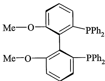
(S)-MeOBiPhep.
