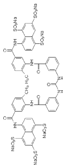
Suramin
