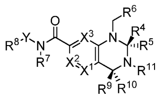
(I-I-IV)-ent 1
