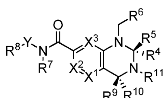
(I-I-IV)-ent 4
