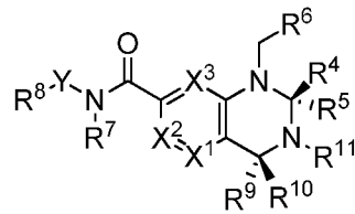
(I-I-IV)-ent 2
