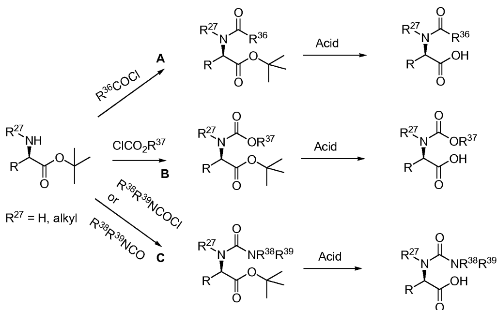
Scheme 13
