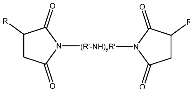
Formula (II)
