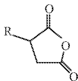
Formula (III)
