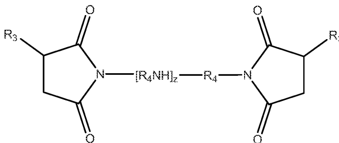
Formula (IV)
