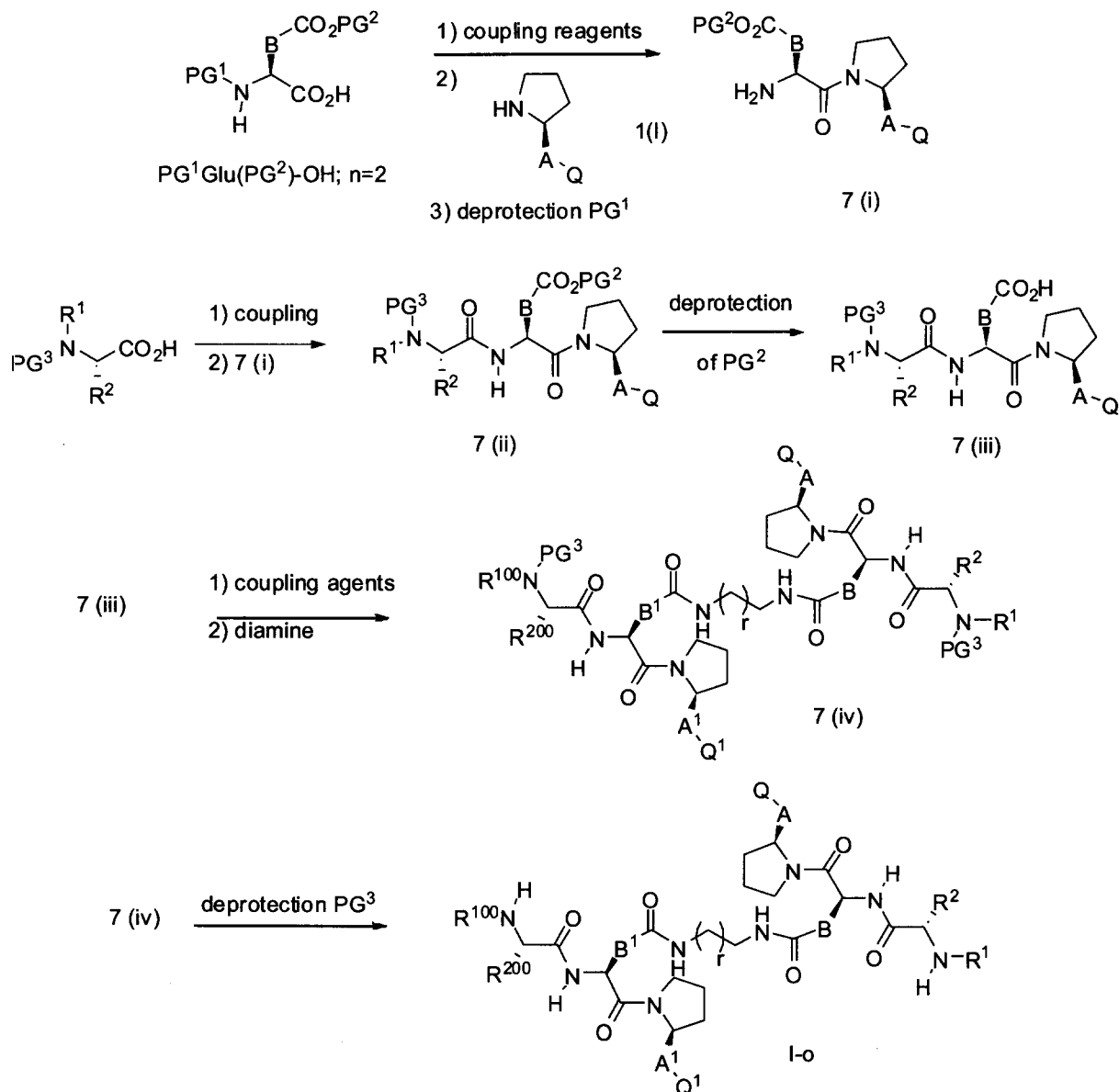
Scheme 7
