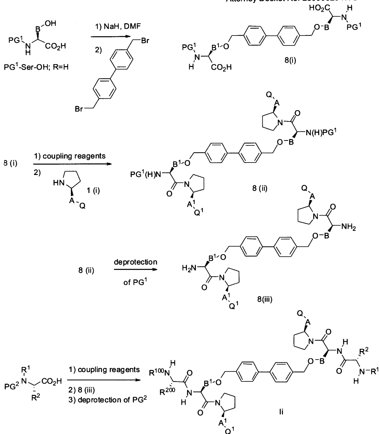
Scheme 8
