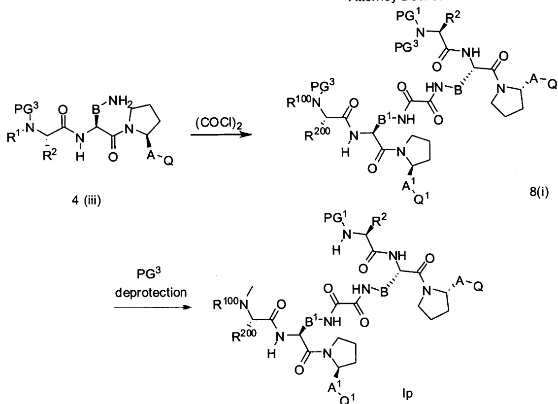
Scheme 9
