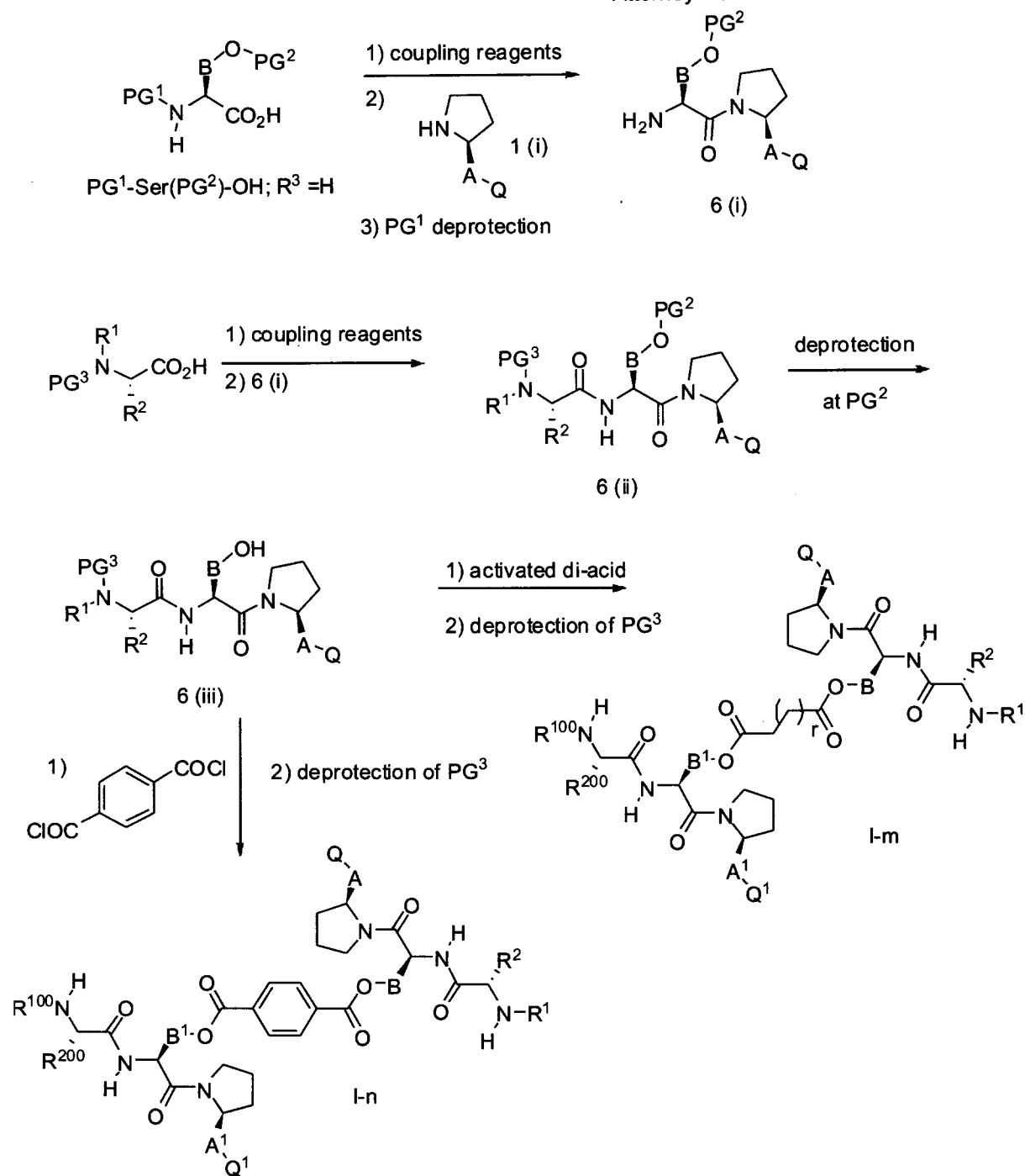
Scheme 6
