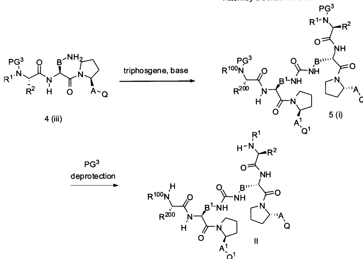
Scheme 5
