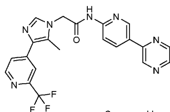
Compound I
